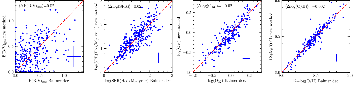
Figure 17. Comparison of E(B-V)_{\text{gas}} (left), SFR( H\alpha ) (left-middle), dust-corrected O_{32} (right-middle), and O/H (right) derived using the new E(B-V)_{\text{gas}} calibration (equation A3; vertical axis) and E(B-V)_{\text{gas}} based on the Balmer decrement (horizontal axis). Red dashed lines show a one-to-one relation, and the mean vertical offset is given in the upper-left corner of each panel.
