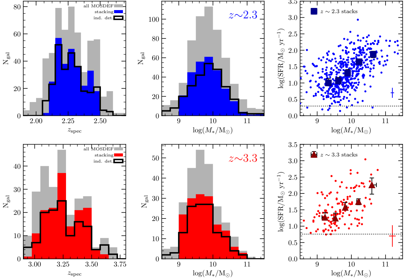
Figure 1. Redshift histogram (left), stellar mass distribution (middle), and SFR vs. M_* for MOSDEF star-forming galaxies at z \sim 2.3 (top) and z \sim 3.3 (bottom). In the left and middle panels, the gray histogram represents all MOSDEF star-forming galaxies in each redshift bin, the black outline shows the subset of individual galaxies with metallicity measurements, and the filled color histogram (blue for z \sim 2.3 , red for z \sim 3.3 ) denotes the stacking sample. In the right panel, individual galaxies are shown as colored dots, while values inferred from stacked spectra in stellar mass bins are presented as colored squares/triangles with error bars. The median uncertainty on M_* and SFR of the individual galaxies is displayed in the lower right corner. The SFR corresponding to the MOSDEF 3\sigma detection limit of H \alpha at z \sim 2.3 and H \beta at z \sim 3.3 is shown by the dotted line in the top and bottom panels, respectively.
