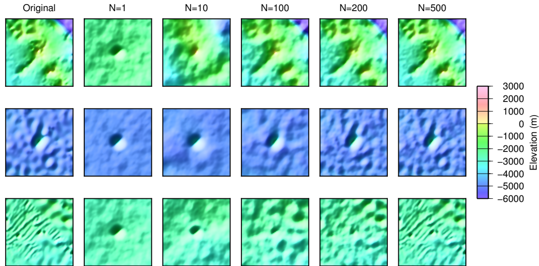
Figure 4. Image reconstruction using principal components. PCA has been performed on a data set containing 1000 square “patches” of bathymetric data, each representing an area of dimension 150 \text{ km} \times 150 \text{ km} , centred upon a seamount (the “training set” used in Valentine et al., 2013). Each patch is comprised of 64 \times 64 samples – thus, each can be seen as a 4096-dimensional object. Three examples from this set are shown here (one per row). In the left-most column we show the original bathymetry for each; then, we present reconstructions of this bathymetry using only the N most significant principal components, for N = 1, 10, 100, 200, and 500 . It is apparent that the large-scale structures within this data set can be represented using only 100–200 dimensions, while around 500 dimensions are required to allow some of the fine-scale structure to be represented, particularly in the third example. This still represents almost an order of magnitude reduction, in comparison to the original, 4096-dimensional, data.
