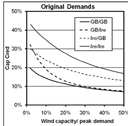
Fig. 2: Capacity credit results from the GB and Irish systems. Sys1/Sys2 denotes demand and conventional generation from Sys1/wind data from Sys2.
