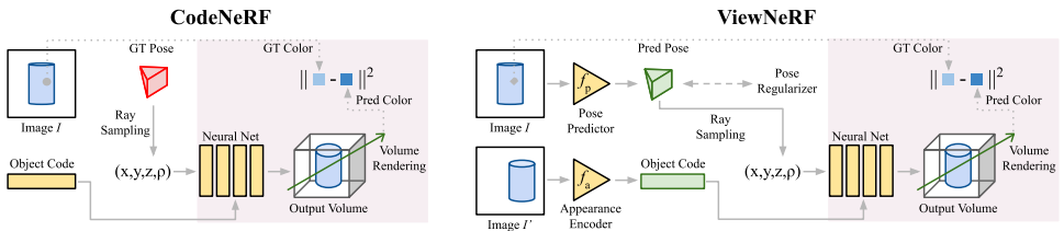
Figure 1: (Left) CodeNeRF [12] requires ground-truth pose information at training time and performs expensive direct optimization for each object appearance code. In practice, CodeNeRF also enforces that the object code for distinct views of the same object are the same which provides some multi-view signal. (Right) In contrast, our ViewNeRF approach is fully self-supervised by making use of a separate pose predictor f_p and appearance encoder f_a that can be applied to any image in a single-shot fashion.
