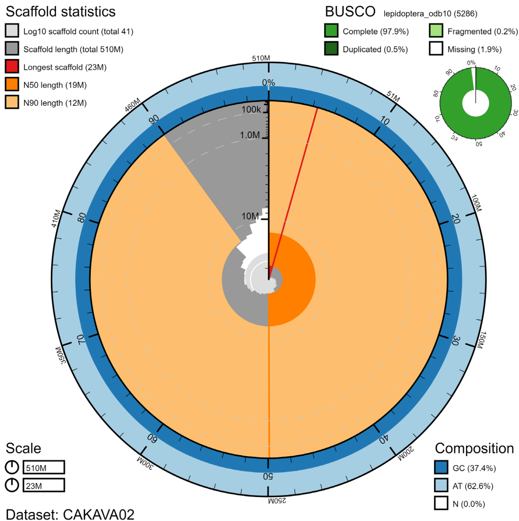
Figure 2. Genome assembly of Erebia ligea , iEreLige1.2: metrics. The BlobToolKit Snailplot shows N50 metrics and BUSCO gene completeness. The main plot is divided into 1,000 size-ordered bins around the circumference with each bin representing 0.1% of the 506,397,422 bp assembly. The distribution of chromosome lengths is shown in dark grey with the plot radius scaled to the longest chromosome present in the assembly (22,722,498 bp, shown in red). Orange and pale-orange arcs show the N50 and N90 chromosome lengths (19,149,538 and 12,368,103 bp), respectively. The pale grey spiral shows the cumulative chromosome count on a log scale with white scale lines showing successive orders of magnitude. The blue and pale-blue area around the outside of the plot shows the distribution of GC, AT and N percentages in the same bins as the inner plot. A summary of complete, fragmented, duplicated and missing BUSCO genes in the lepidoptera_odb10 set is shown in the top right. An interactive version of this figure is available at https://blobtoolkit.genomehubs.org/view/iEreLige1.2/dataset/CAKAVA02/snail .
