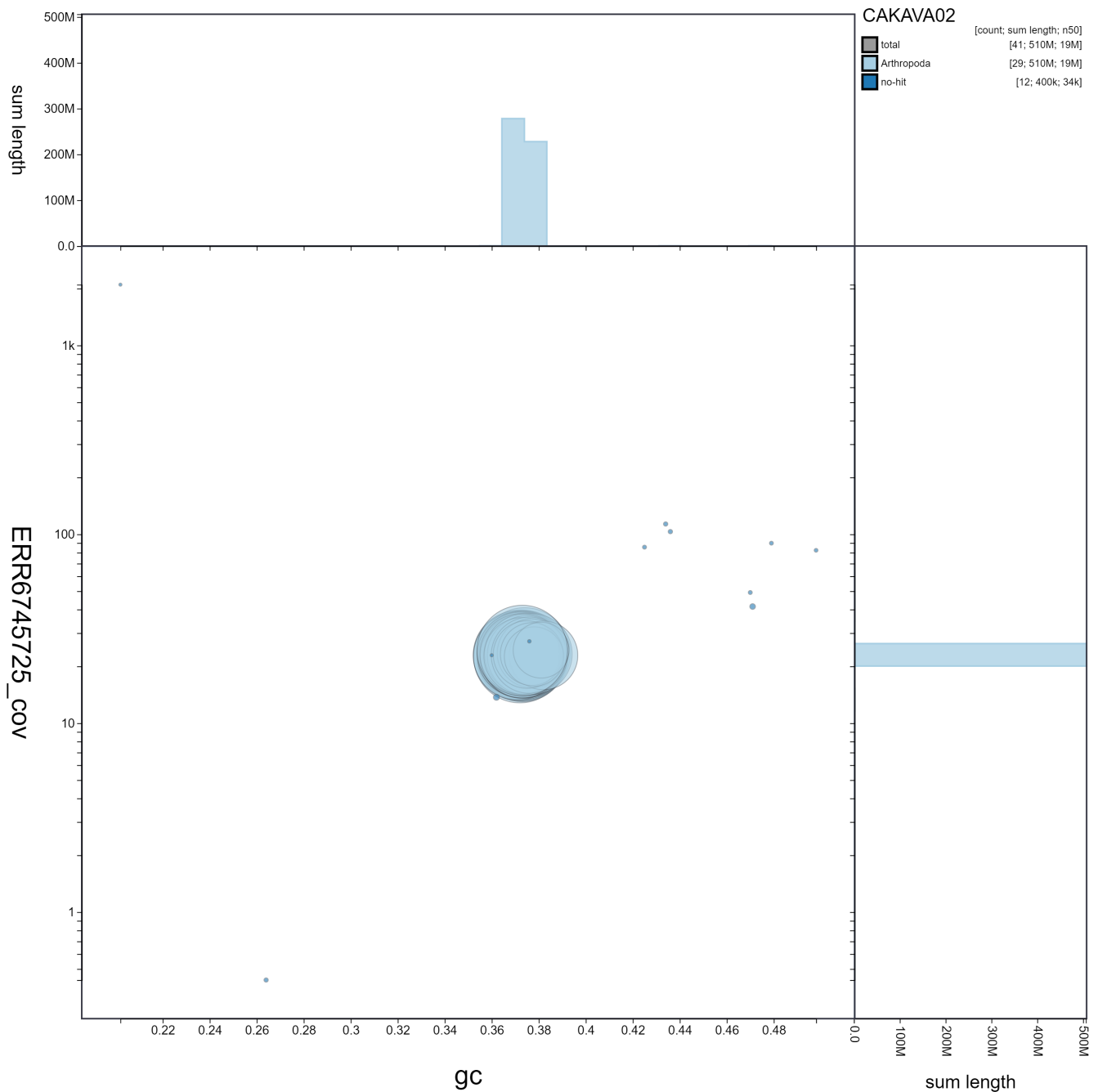
Figure 3. Genome assembly of Erebina ligea , iEreLige1.2: GC coverage. BlobToolKit GC-coverage plot. Scaffolds are coloured by phylum. Circles are sized in proportion to scaffold length. Histograms show the distribution of scaffold length sum along each axis. An interactive version of this figure is available at https://blobtoolkit.genomehubs.org/view/iEreLige1.2/dataset/CAKAVA02/blob .
