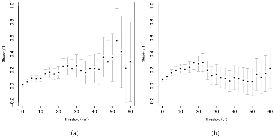
Figure 4. Maximum likelihood estimates of the shape parameters and corresponding 95% confidence intervals over a grid of thresholds; left and right tails are in (a) and (b), respectively.
