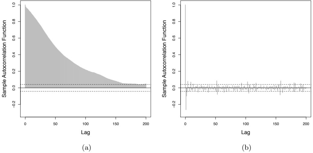
Figure 2. Correlogram for (a) the weekly number of unemployment insurance claims in the US (initial claims), for the original data and (b) the data in first differences.
