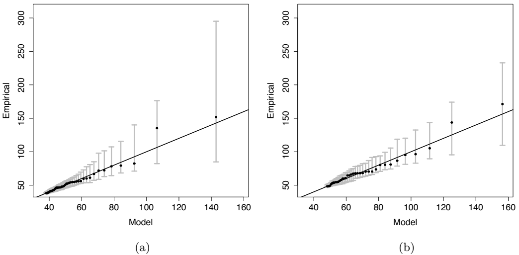
Figure 5. Quantile plots for the fits of the peaks over threshold model and corresponding simulated 95% confidence intervals corresponding to: (a) left tail; (b) right tail.
