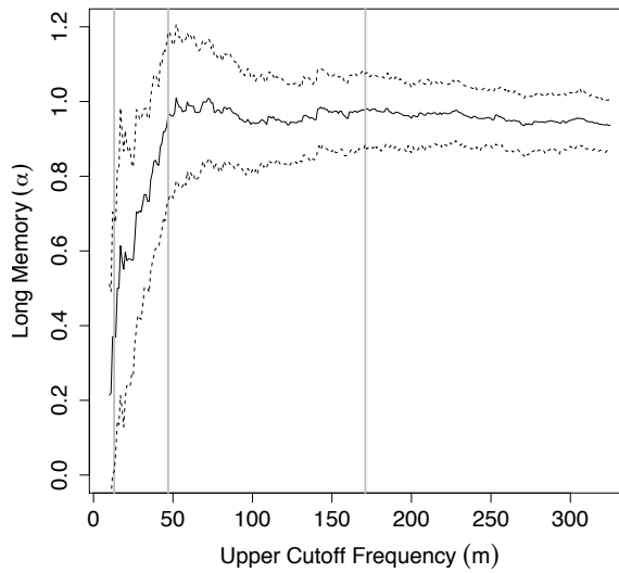
Figure 3. The solid line represents the GPH estimates of \alpha with m ranging from 10 up to n^{3/4} ; the gray vertical lines correspond to n^{1/3} , n^{1/2} , and n^{2/3} , and the dashed lines represent 95% pointwise confidence bands, which were obtained by the bootstrap.
