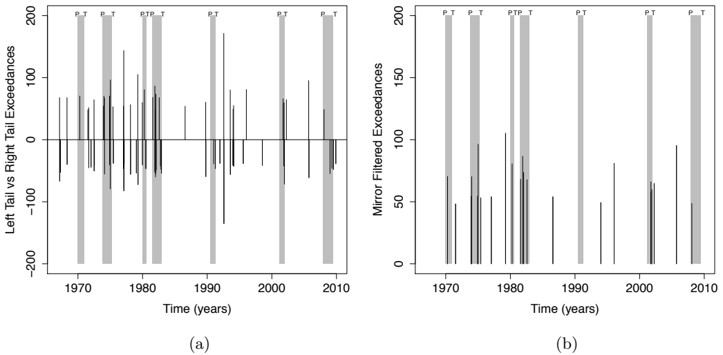
Figure 8. (a) Mirror plot; (b) Mirror filtered exceedances.
