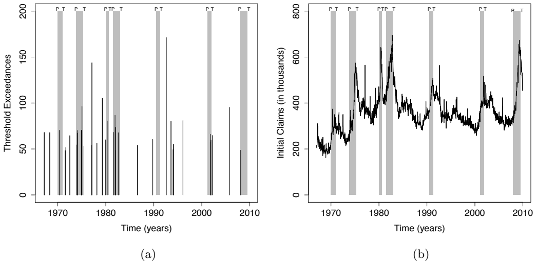
Figure 7. (a) Threshold exceedances; (b) Weekly number of unemployment insurance claims in the US (initial claims). Shaded areas represent the US economic activity contractions dated by the Business Cycle Dating Committee of the NBER.
