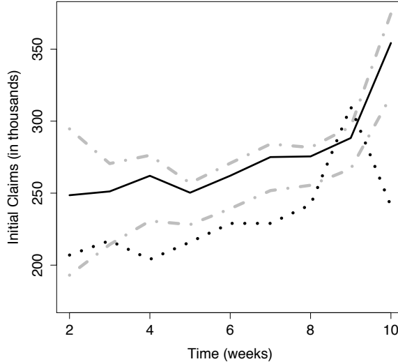
Figure 6. The solid line represents the dynamic threshold constructed according to (8); the 95% pointwise confidence bands constructed by the bootstrap, and the initial claims are respectively represented by the dashed–dotted and dashed lines.
