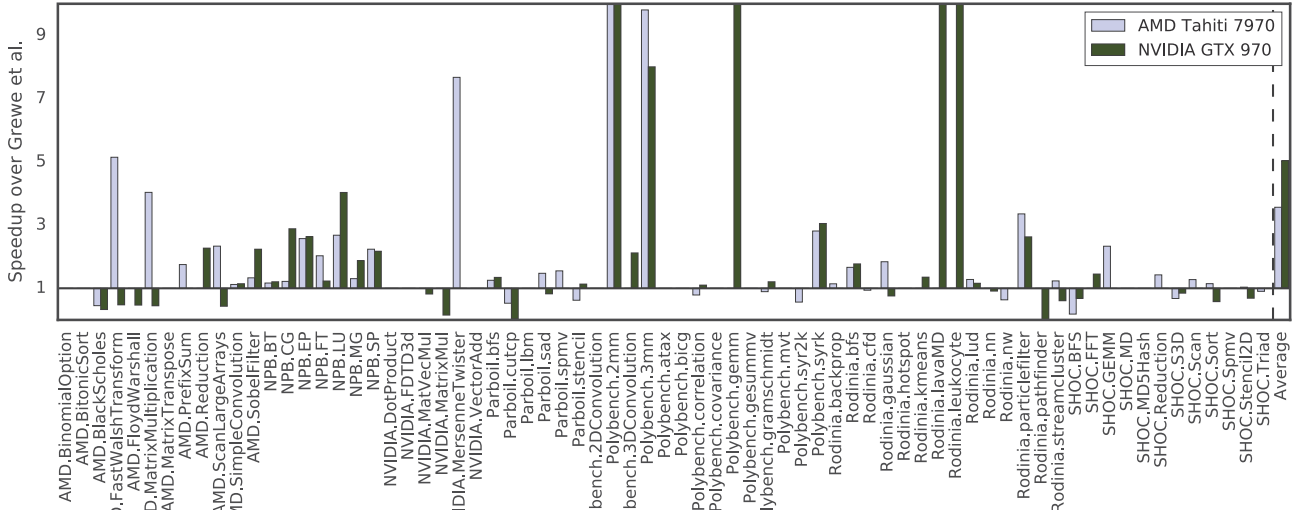
Figure 8. Speedups of predictions using our extended model over Grewe et al. on both experimental platforms. Synthetic benchmarks and the additional program features outperform the original predictive model by a factor 3.56\times on AMD and 5.04\times on NVIDIA.
