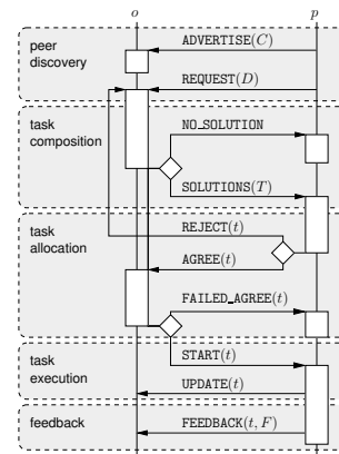
Figure 1: Team task protocol, adapted from [15]. Swimlanes represent peer roles, boxes their internal processing steps, and diamonds choice points.
