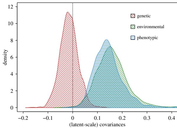
Figure 2. Posterior distributions of the estimates of components of covariance between nestling mass and juvenile survival in superb fairy-wrens (from model I, table 1). Red diagonal hashed lines indicate the additive genetic covariance, green diagonal lines indicate the environmental (non-genetic) covariance (defined as in S2) and blue horizontal lines indicate the phenotypic covariance. Survival was modelled as a threshold trait with a probit link function, so the parameter estimates are on the latent scale. Despite the positive phenotypic covariance and additive genetic variance for both traits (electronic supplementary material, figure S1), there was little support for positive additive genetic covariance.
