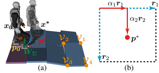
Fig. 3: (a) Variables definition of the oracle. \mathbf{x}_0 and \mathbf{p}_0 are the initial CoM state and initial swing-foot position. \mathbf{x}^* and \mathbf{p}^* are the target CoM state and the contact location respectively. Purple patches are initial contact surfaces, while blue patches are for future steps. Contact surfaces are modeled by their vertices \mathcal{V}_i . Spatial terms are defined in the contact frame \mathcal{W}_\Sigma established at the non-swing foot. (b) The target contact location \mathbf{p}^* is represented as the vector sum of \alpha_1 \mathbf{r}_1 and \alpha_2 \mathbf{r}_2 , which scale along the contact surface borders \mathbf{r}_1, \mathbf{r}_2 \in \mathbb{R}^3 with the proportion defined by \alpha_1, \alpha_2 \in [0, 1] .
