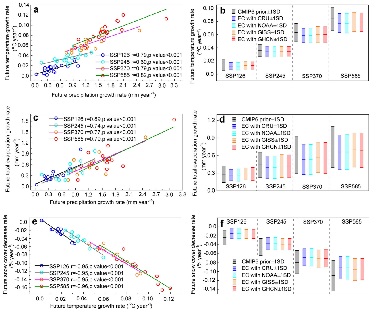
Fig. 3 Emergent constraint (EC) on future temperature, total evaporation, and snow cover fraction changes in Asia after applying the constrained future precipitation growth rate. a is the constraint relation between the future growth rate of precipitation ( \text{mm year}^{-1} ) and the future growth rate of temperature ( ^{\circ}\text{C year}^{-1} ) under SSP126, SSP245, SSP370, and SSP585 emission scenarios; (b) is the best estimate \pm one standard deviation of the original and constrained future annual growth rate of temperature when the constrained precipitation is derived from the HadCRUT4, NOAA, GISS, and GHCN observational data sets. Similarly, (c, e) present constraint relationships between future annual precipitation and total evaporation growth rates ( \text{mm year}^{-1} ), and between future annual temperature and snow cover fraction ( \% \text{ year}^{-1} ) growth rates, respectively, with the snow-free regions of Asia excluded. d, f present the best estimate \pm one standard deviation for future annual total evaporation and for future annual loss in snow cover fraction, respectively. Please also refer to Section 5 of Supplementary Text and Supplementary Fig. 28 for comparison between the different changing directions of the constrained results.
