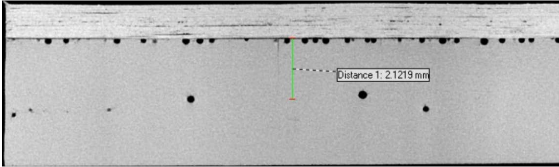
Figure 11. A 2 mm deep microcrack through the thickness of the polymer liner region in a [0/90/0/90]_s CF/PEEK to PEEK 150PF LATP laminate after 50 cycles.
