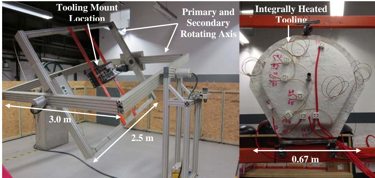
Figure 1. The biaxially rotating arms of the rotational moulding rig with the integrally heated tooling also pictured.
