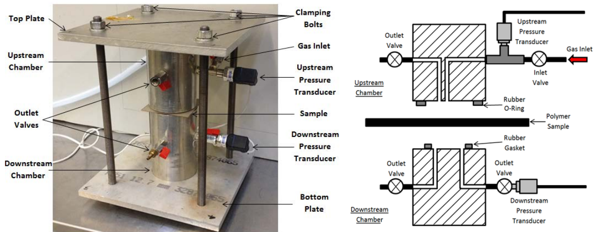
Figure 2. The permeability test rig used along with a schematic of the internal structure.
