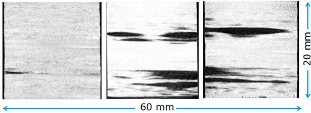
Figure 9. X-Ray CT images of debonding regions between the CF/PEEK tape and the PEEK 150PF liner surface highlighted by the darker regions signifying air gaps in the bond region.
