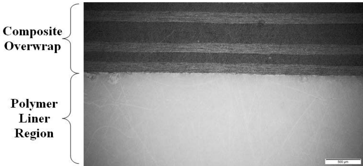
Figure 8. Microscopy image of the liner-overwrap cross section in a PEEK 150PF liner overwrapped with 8 layers of CF/PEEK tape.
