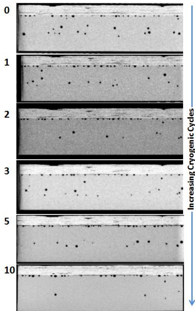
Figure 10. Cross sectional X-Ray CT images of a cryogenically cycled [0/90/0/90]_s CF/PEEK to PEEK 150PF LAMP laminate before cycling and after 1, 2, 3, 5 and 10 cycles with no micro-cracks present.
