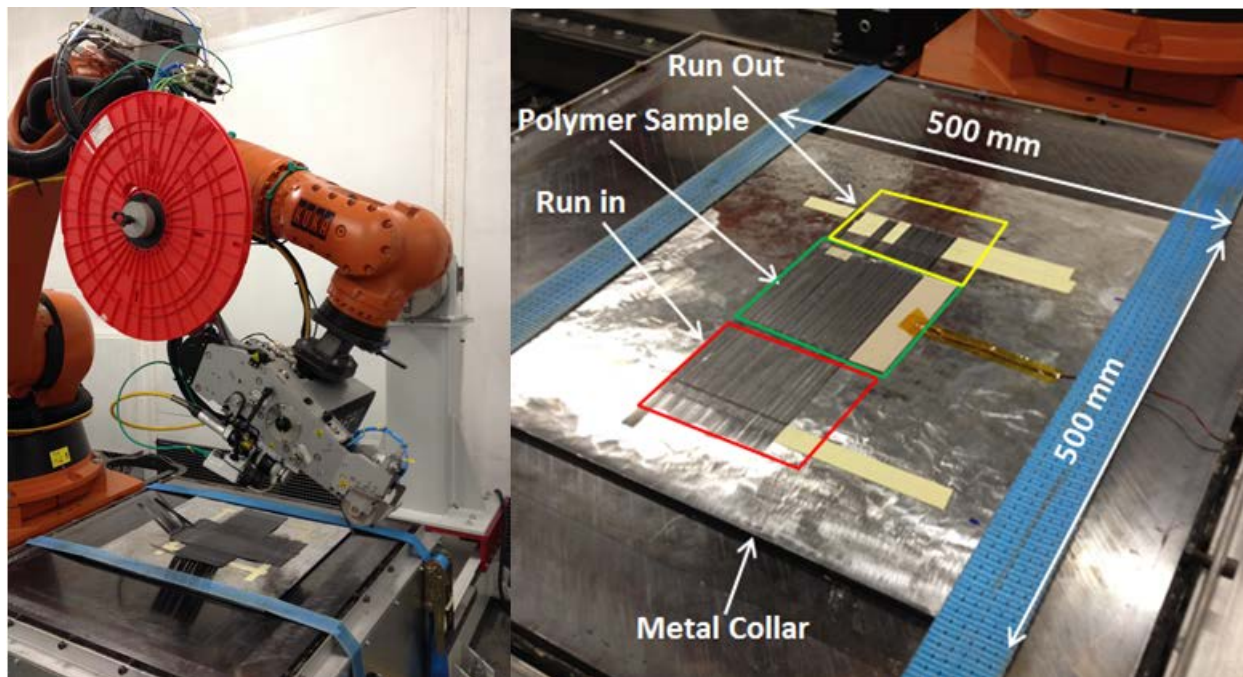
Figure 3. The LATP unit used and the overwrapping methodology for carbon fibre thermoplastic tape laying over polymer liner samples.
