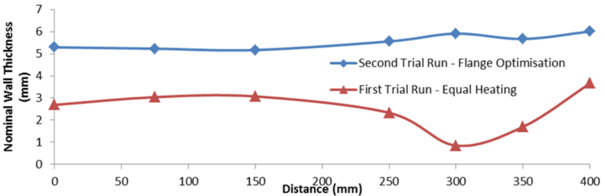
Figure 5. Wall thickness distributions along the demonstrator length for two different heating cycles with significant differences visible at the parting line (300 mm mark).
