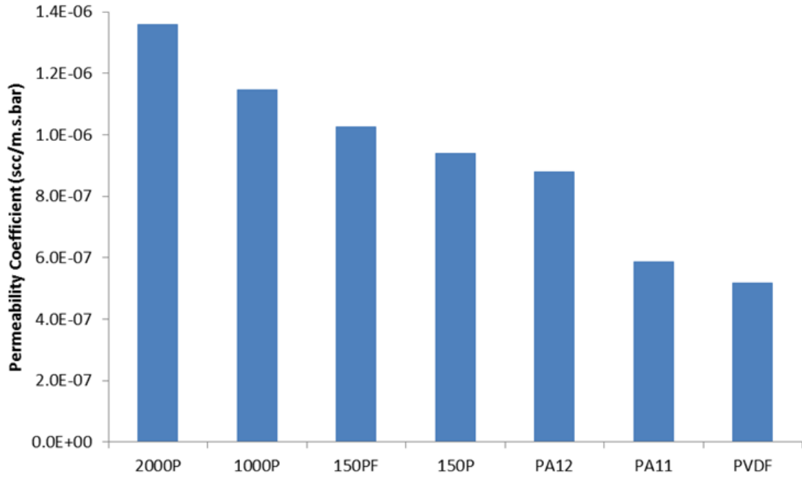
Figure 6. Permeability coefficient results for all polymer materials tested.
