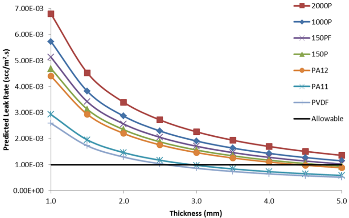
Fig. 7. Predicted leak rates for a 1 m 2 area of each material with a 5 bar pressure difference for varying liner thicknesses.
