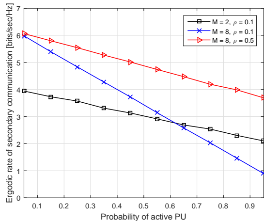
Fig. 7. Ergodic rate of RX s vs. primary activity profile (optimized hybrid CR system), for different values of antenna number, M , and correlation factor, \rho , when \tilde{\mathcal{P}}_{\text{out}} = 2 \times 10^{-2} .
