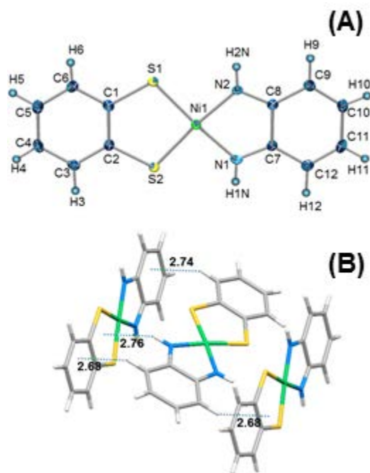
Figure 1. (A) Ortep diagram of [Ni(bdt)( o -phen)] ( 1 ) with atom labeling and thermal ellipsoids drawn at the 50% probability level; (B) close C—H \cdots \pi and N—H \cdots \pi interactions between adjacent molecules.
