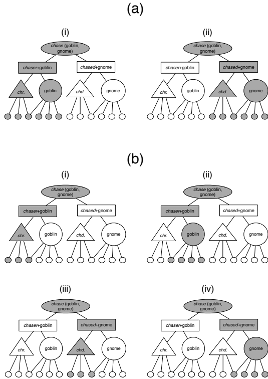
Figure 2. Dynamic binding in LISA and DORA. (a) Binding in LISA. (i) To bind the role chaser to goblin, units coding for the chaser role and goblin (as well as those coding conjunctively for chaser+goblin ) fire. (ii) To bind chased to gnome, units coding for the chased role and gnome (as well as those coding conjunctively for chased+gnome ) fire. (b) Binding in DORA. (i-ii) To bind the role chaser to goblin, units coding for the chaser role (as well as those coding conjunctively for chaser+goblin ) fire, followed by the units coding for goblin (as well as those coding conjunctively for chaser+goblin ). (iii-iv) To bind the role chased to gnome, units coding for the chased role (as well as those coding conjunctively for chased+gnome ) fire, followed by the units coding for gnome (as well as those coding conjunctively for chased+gnome ).
