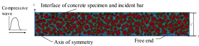
Figure 10: Mesoscale model configuration
