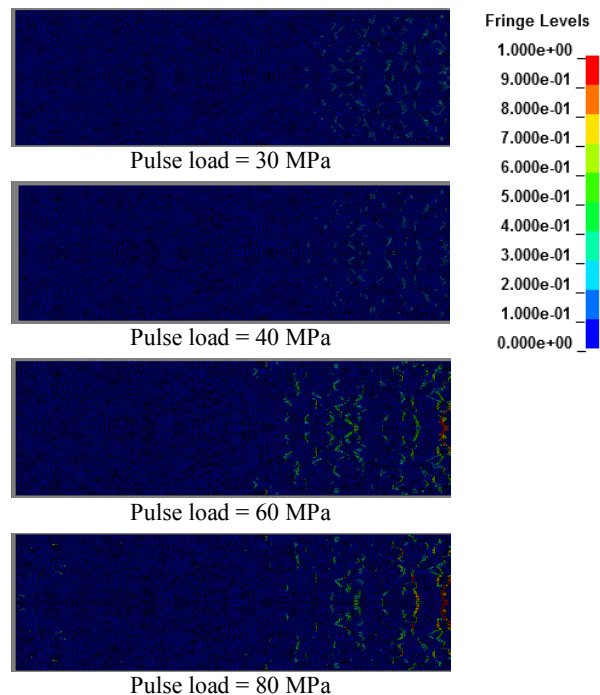
Figure 12: Distribution of tensile damage in the mesoscale model under different loading & rates
