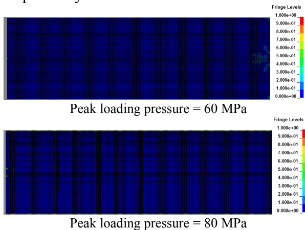
Figure 9: Damage values representing the fracture patterns under increased peak imposed pressure (and loading rate).
