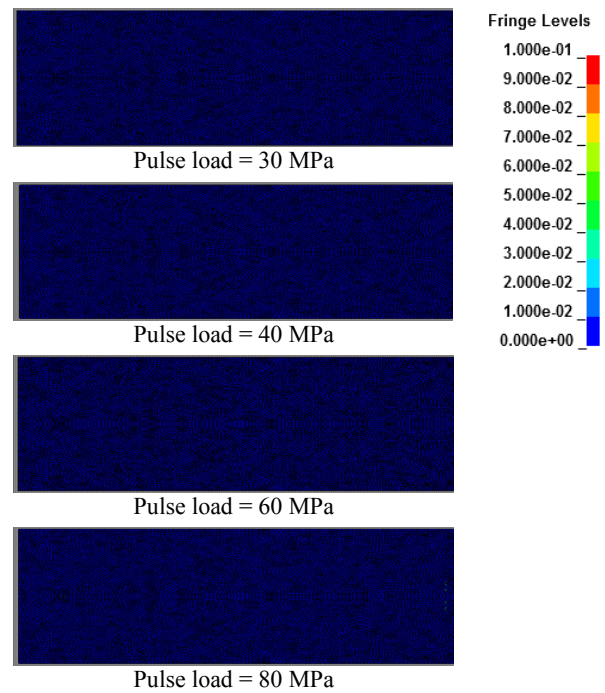
Figure 11: Macro crack patterns (represented by final plastic strain) of the mesoscale model under different loading & rates
