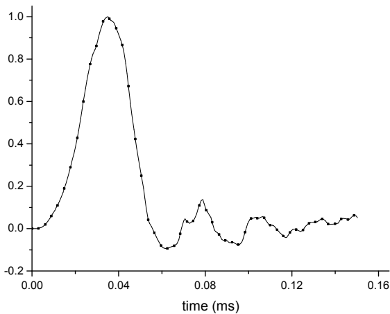
Figure 4: Typical pressure input as stress boundary.
