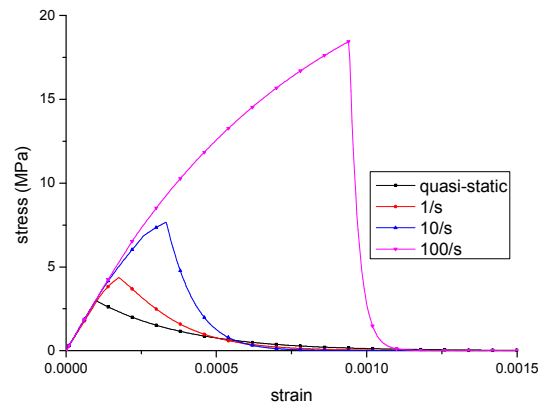
Figure 5: Tensile stress-strain curves generated by the material model
