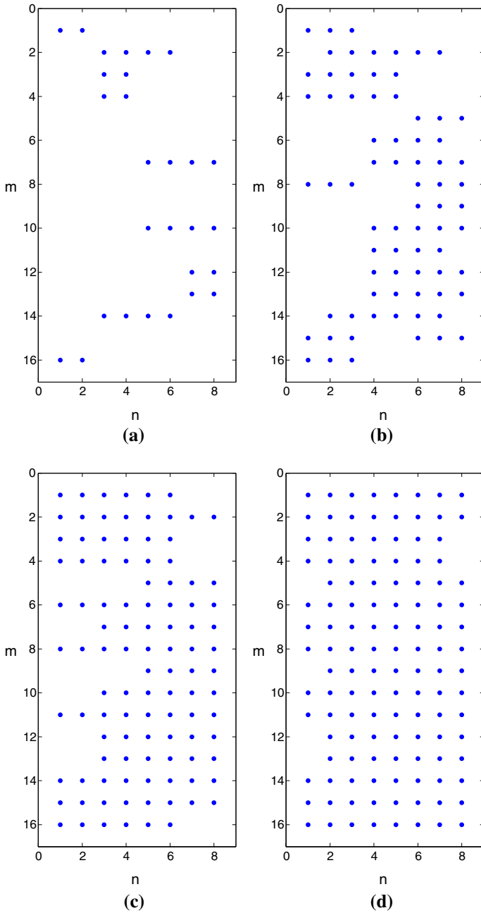
Fig. 3 Sparsity pattern of four examples of matrix A , the Givens rotations G and G_2 are explained in Sect. 4.1 and 4.2. a A = (PGP)\Sigma G^T . b A = (P\tilde{G}_2\tilde{G}P)\Sigma(G_2G)^T . c A = (P\tilde{G}\tilde{G}_2\tilde{G}P)\Sigma(GG_2G)^T d A = (P\tilde{G}_2\tilde{G}\tilde{G}_2\tilde{G}P)\Sigma(G_2GG_2G)^T
