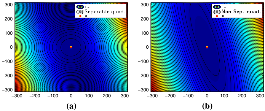
Fig. 2 Demonstration of the contours of two different types of function Q_\tau , which locally approximate function f_\tau at point x . In the left figure , function Q_\tau is a simple separable quadratic for which, H = \lambda_{max}(A^T A)I_n in (4), that is frequently used in first-order methods. In the right figure , function Q_\tau is a non separable quadratic (9) which is used in some of the second-order methods. a Separable quadratic. b Non separable quadratic
