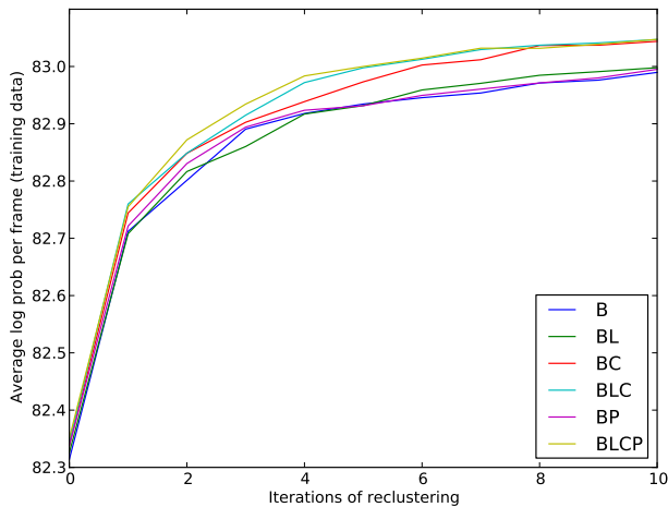
Figure 3: Likelihood of training data given model during voice-building.
