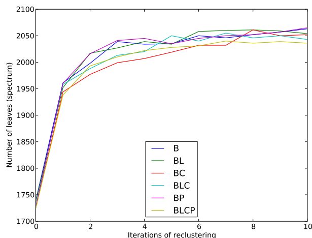
Figure 1: Model size during voice-building: spectral envelope.
