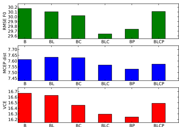
Figure 4: Results of objective evaluation.
