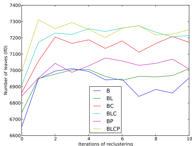
Figure 2: Model size during voice-building: log F0.
