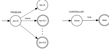
Figure 6: continuous problem with the goal loc \neq 0
