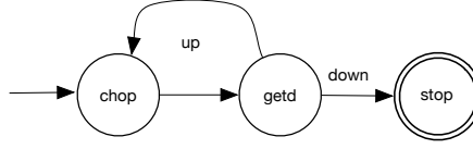
Figure 2: controller for chopping a tree of unknown non-zero thickness d , by means of a binary sensing action getd
