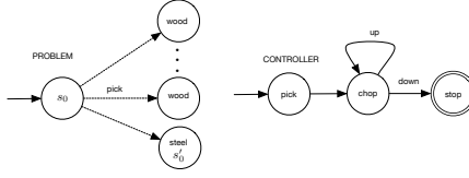
Figure 5: wood and steel trees
