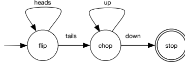
Figure 7: controller for flip and chop
