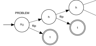
Figure 4: coin flip problem where after infinitely many heads, a tails can still be observed
