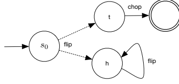
Figure 9: bad flip and chop problem
