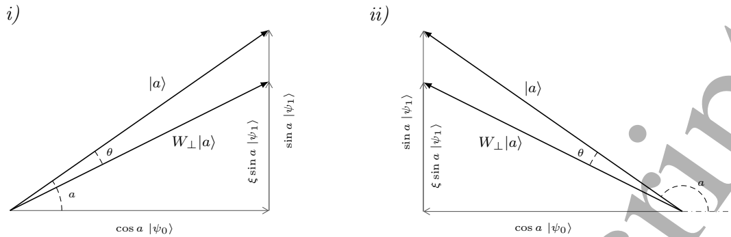
Figure 3: Geometric relation between the angle a before weak measurement and the offset \theta(a, \kappa) after measuring outcome \perp . The construction is provided when i) a is in the first quadrant and when ii) a is in the second quadrant.
