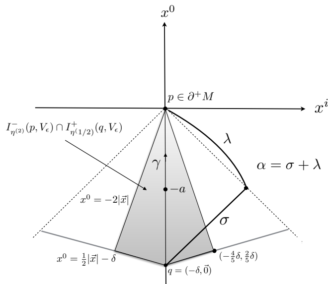
Figure 1: \lambda(-a) lies to the future of the wide cone and is on or outside the “narrow” cone.
