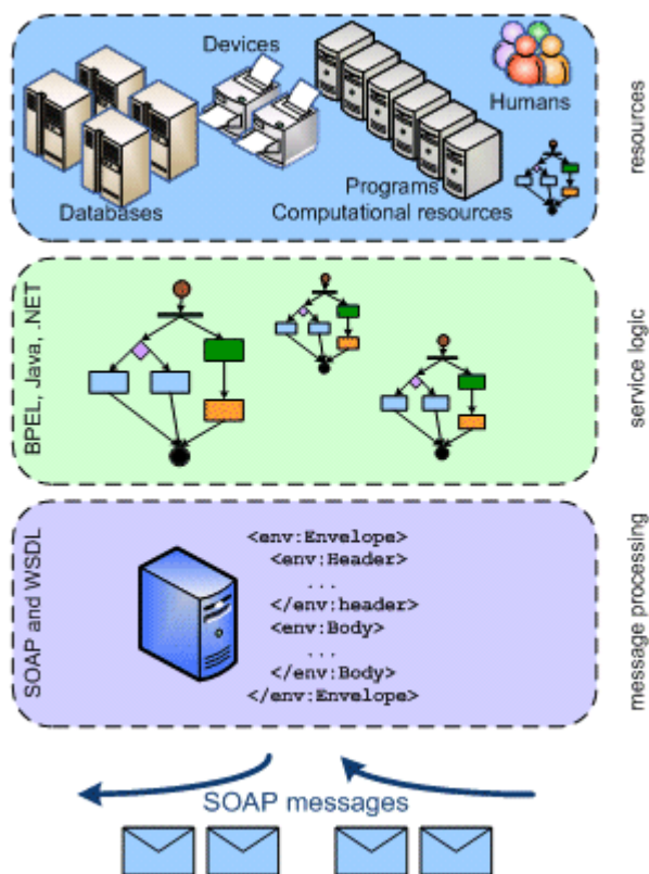
Figure 2 Anatomy of a Web Service
