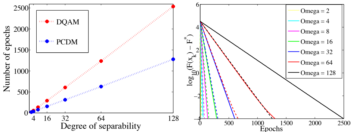
Figure 1: The left plot shows the number of epochs (a full sweep through the data, i.e., all i = 1, \dots, n blocks of x are updated in one epoch) needed to solve the problem as a function of the degree of separability \omega . PCDM requires far fewer epochs to reach the stopping condition compared with DQAM. The right plot shows the number of epochs versus the decrease in the function value. The colours correspond to different values of \omega , with dotted lines corresponding to PCDM and solid lines corresponding to DQAM. Again, this plot shows the superiority of PCDM and also shows the linear convergence behaviour of the algorithms.
