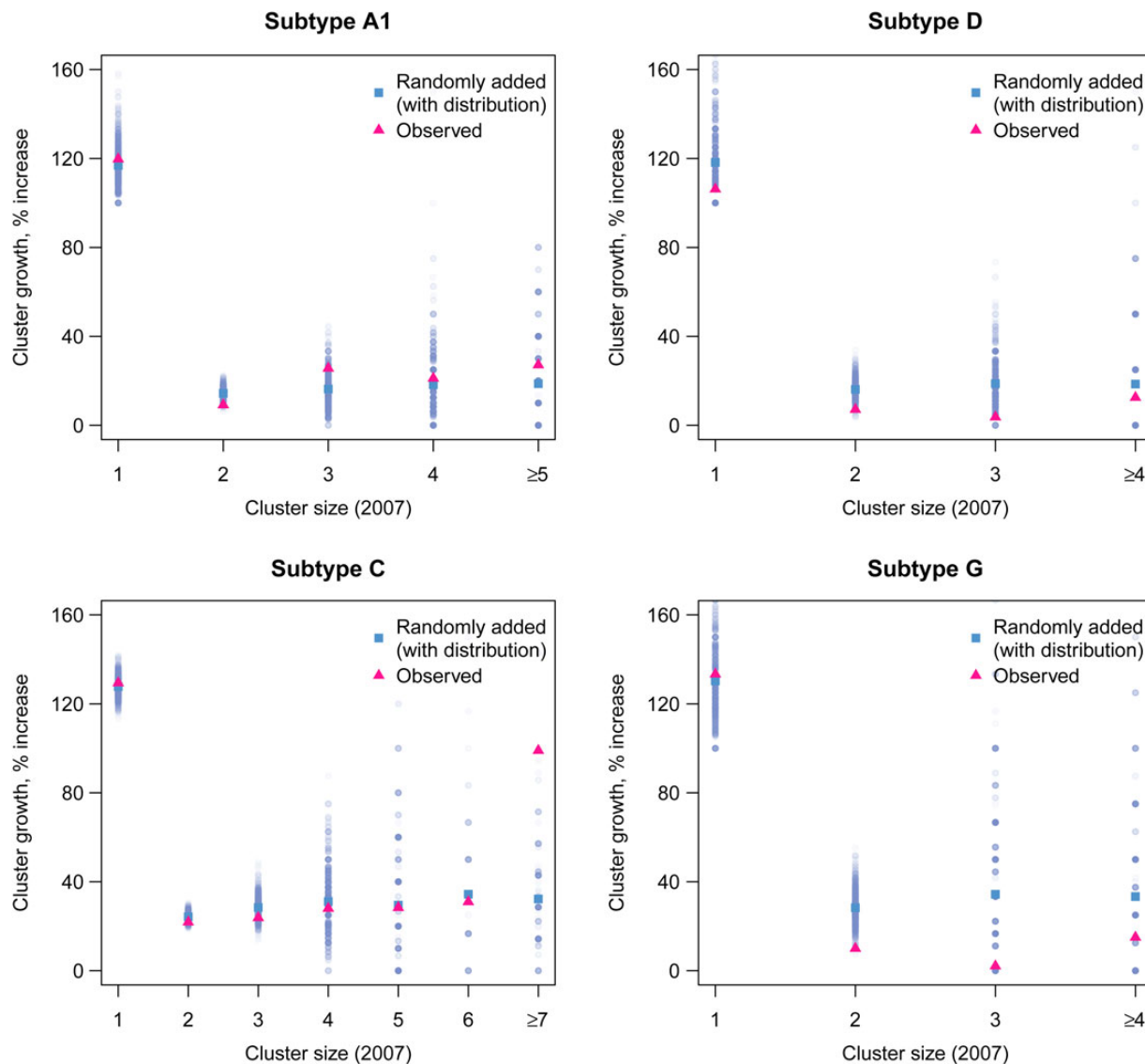
Figure 2. Cluster growth according to initial cluster size in 2007. For each cluster identified in 2009 containing at least 1 sequence collected before 2007, cluster growth was calculated as the number of new sequences divided by the number of old sequences (pink or black triangles). In parallel, we conducted simulations to generate expected cluster growth according to initial cluster size (blue or gray triangles). Data are from 1000 simulations, and mean values and distributions are shown. This figure is available in black and white in print and in color online.
