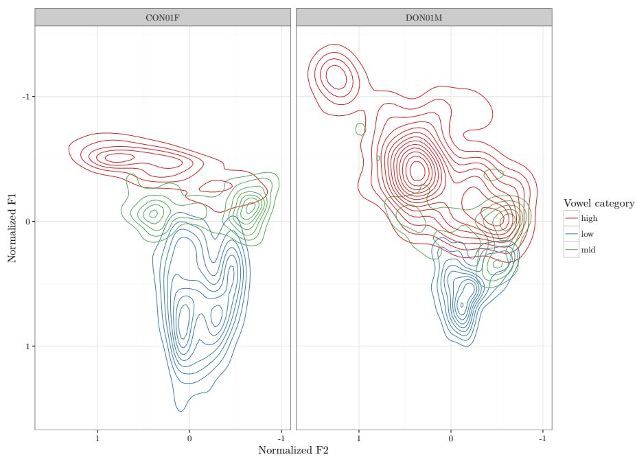
Figure 2: Density of distribution, midpoints, 3-category model
