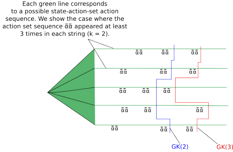
Figure 8: This figure illustrates the notion that the action set sequence \bar{\alpha}\bar{\alpha} appears 3 times for all strings. The sets GK(m) are defined in (7).
