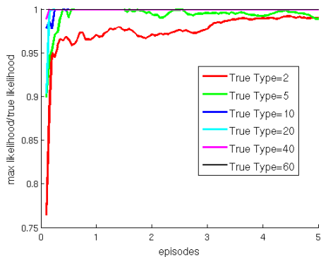
Figure 4: The ratio of the maximum-likelihood type and posterior and the true type in BEAT, averaged over all population-diversity trials in our experiments. The user is simulated.
