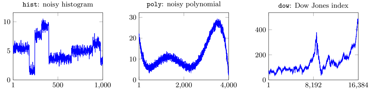
Figure 1: Data sets for the offline histogram approximation experiments. (left) hist is a histogram consisting of 10 pieces contaminated with Gaussian noise ( n = 1000 ). (middle) poly is a degree 5 polynomial, also contaminated with Gaussian noise ( n = 4000 ). (right) dow is a time series of Dow-Jones Industrial Average (DJIA) daily closing values ( n = 16384 ).
