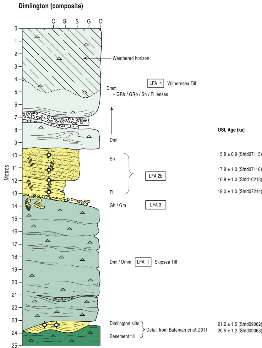
Fig. 5. Composite vertical profile log for the LGM typesite at Dimlington modified from Evans and Thomson (2010) with detail of Dimlington silts and Basement Till taken from Bateman et al. (2011). OSL sample locations and ages of this study shown in appropriate stratigraphic position.
