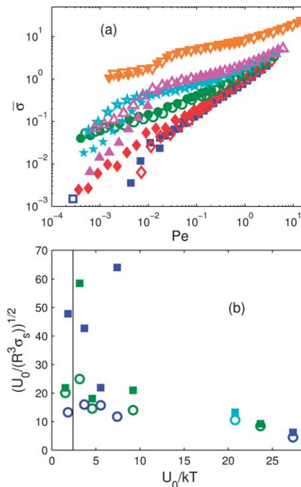
Fig. 5 (a) Normalized flow curves for \phi = 0.45 , R = 138 nm at various attraction strengths -U_0 = 0, 2.3, 4.7, 7, 9.4 , and 34.6 k_B T (resp. \blacksquare, \blacklozenge, \bullet, \blacktriangle, \blacktriangledown ), open and close symbols decreasing and increasing shear rates respectively. (b) \sqrt{|U_0|R^{-3}\sigma_s^{-1}} versus |U_0|/k_B T for R = 138 nm, \phi = 0.45 and various polymer concentrations. The open circles use the values of the yield stress going from high to low shear rates, the full squares are the values going from low to high shear rates, the continuous line marks the gel transition. Rheology data are taken with smooth surfaces.
