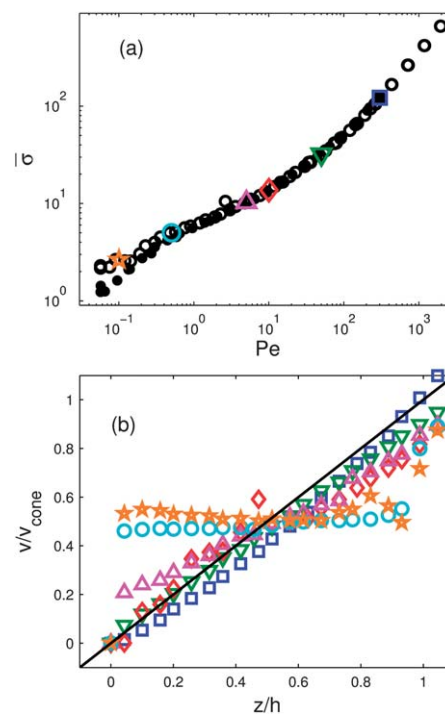
Fig. 2 (a) Flow curves for R = 650 nm, \phi = 0.4 , and U_0 = -20 k_B T in density- and index-matching solvent with coated cone and plate, for decreasing ( \square, \circ ) and increasing ( \bullet ) \dot{\gamma} . Other symbols show where the velocity profiles in (b) were taken. (b) Velocity profiles normalized by the cone velocity versus the position in the gap for \dot{\gamma} = 30 s -1 ( \square ), \dot{\gamma} = 5 s -1 ( \nabla ), \dot{\gamma} = 1 s -1 ( \diamond ), \dot{\gamma} = 0.5 s -1 ( \triangle ), \dot{\gamma} = 0.05 s -1 ( \circ ), and \dot{\gamma} = 0.01 s -1 ( \star ).
