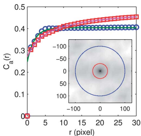
Fig. 10 C_a(r) for \dot{\gamma} = 1 \text{ s}^{-1} (○) and \dot{\gamma} = 30 \text{ s}^{-1} (◻), the magenta and green lines are the respective fit by eqn (4). Inset C_a(x, y) at \dot{\gamma} = 1 \text{ s}^{-1} , the blue dots mark the points used for r = 100 , the red dots for r = 30 .
