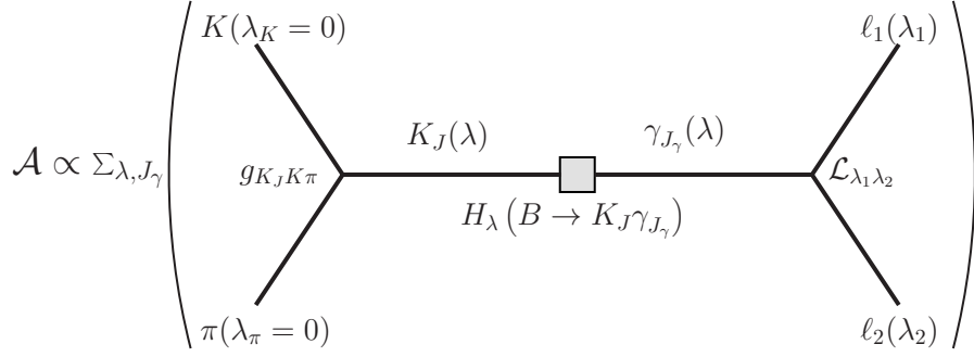
Figure 2: A diagrammatic interpretation of the process, Eq. (20), used to set up the formalism. The decay to two leptons is treated as being mediated by an effective particle \gamma_{J_\gamma} of spin J_\gamma . The factor g_{K_J K \pi} has no dependence on helicities and depends only on the dynamics of the K^* decay.
