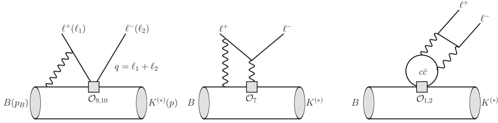
Figure 3: Examples of virtual QED corrections to B \rightarrow K \ell^+ \ell^- , where either a photon is exchanged between the decaying b -quark and a final state lepton, with effective operators \mathcal{O}_{9,10} (left) or \mathcal{O}_7 (middle), or a second photon is emitted by the charm loop (right). Other topologies relevant for higher moments include the interaction of the leptons with the spectator as well as the B - and K^{(*)} -meson.
