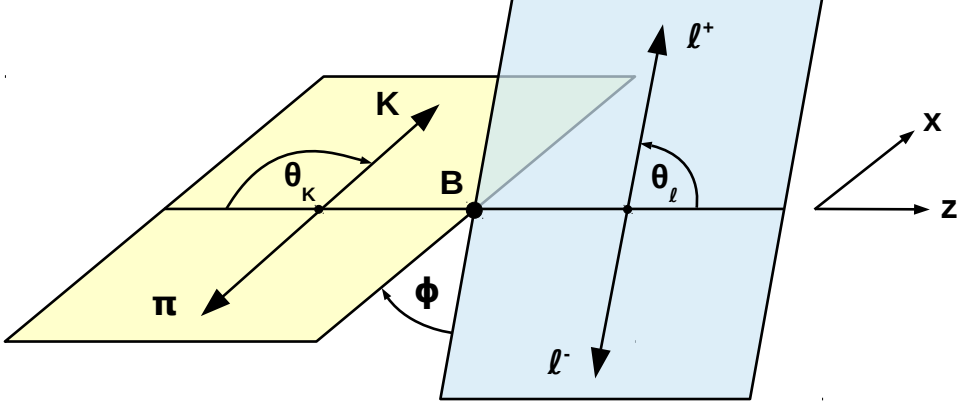
Figure 1: The two decay planes and the definition of the angles used in the calculations. The z-axis is aligned along the flight direction of the momentum of the lepton pair. The conventions are the same as used by the LHCb collaboration in [31]. Alternative conventions, as used in the theory community, are given in Eq. (12), and their impact on the sign of the angular functions J_i is given in Tab. 3.
