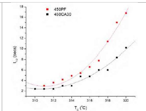
Figure 20: Comparison of half-time values for unreinforced PEEK (450PF in red) and CF/PEEK (450CA30 in black) [22].
