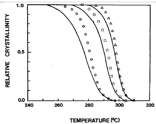
Figure 34: Comparison of the experimental data (points) with the calculated values (lines) from using only the heterogeneous term kNt^n in Eqn. (4.18) at the cooling rates (○) 50°C/min, (□) 20°C/min, and (△) 10°C/min [87].
