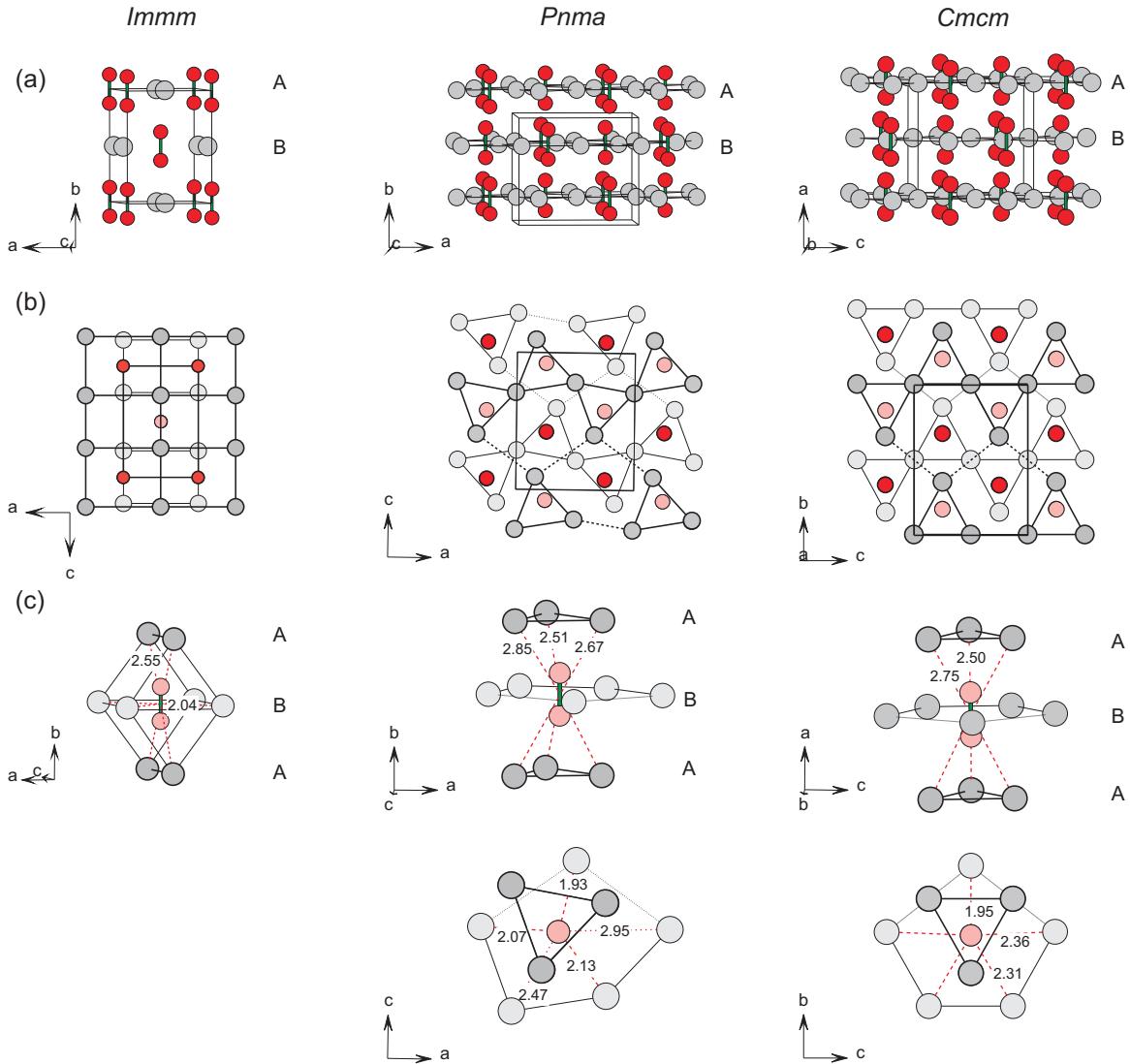
FIG. 7. (Color online) (a) Crystal structures of Immm , Pnma , and Cmcm Li_2C_2 represented as layers consisting of planar nets formed by Li ions, which are centered by perpendicularly oriented dumbbell units. Li ions are shown as light gray circles and C atoms as red circles. Layers are stacked with an AB sequence in the dumbbell direction, as described in the text. (b) View of the structures along the layer stacking direction. A-type layers are distinguished by bold lines. B-type layers by thin lines and pale colors. (c) Coordination of C_2 dumbbells within the three phases. The numbers indicate the distances between the dumbbell center and surrounding Li ions in Å (referring to DFT optimized structures at 20 GPa).
