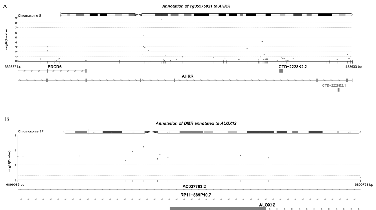
Fig. 3 a Genomic location of cg05575921. b Genomic location of CpGs annotated to DMR ALOX12
