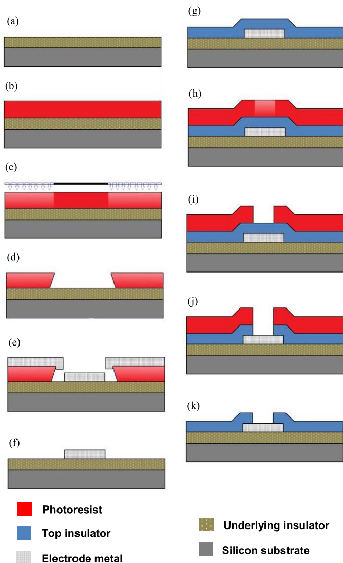
Fig. 2. Cross-sections of the fabrication procedure used to produce the microelectrodes. (a) An underlying insulator of \text{SiO}_2 or Si-rich \text{SiN} is grown/deposited on a silicon wafer. (b)-(f) The tungsten electrode metal area is then defined using a pattern and lift-off technique. (g) The top insulator of Si-rich \text{SiN} or \text{Si}_3\text{N}_4 is then deposited. (h)-(i) The areas to become the microelectrode and contact pad are defined using photolithography. (j) The exposed areas are then etched to expose the electrode metal. (k) The resist is then stripped and the device is completed.
