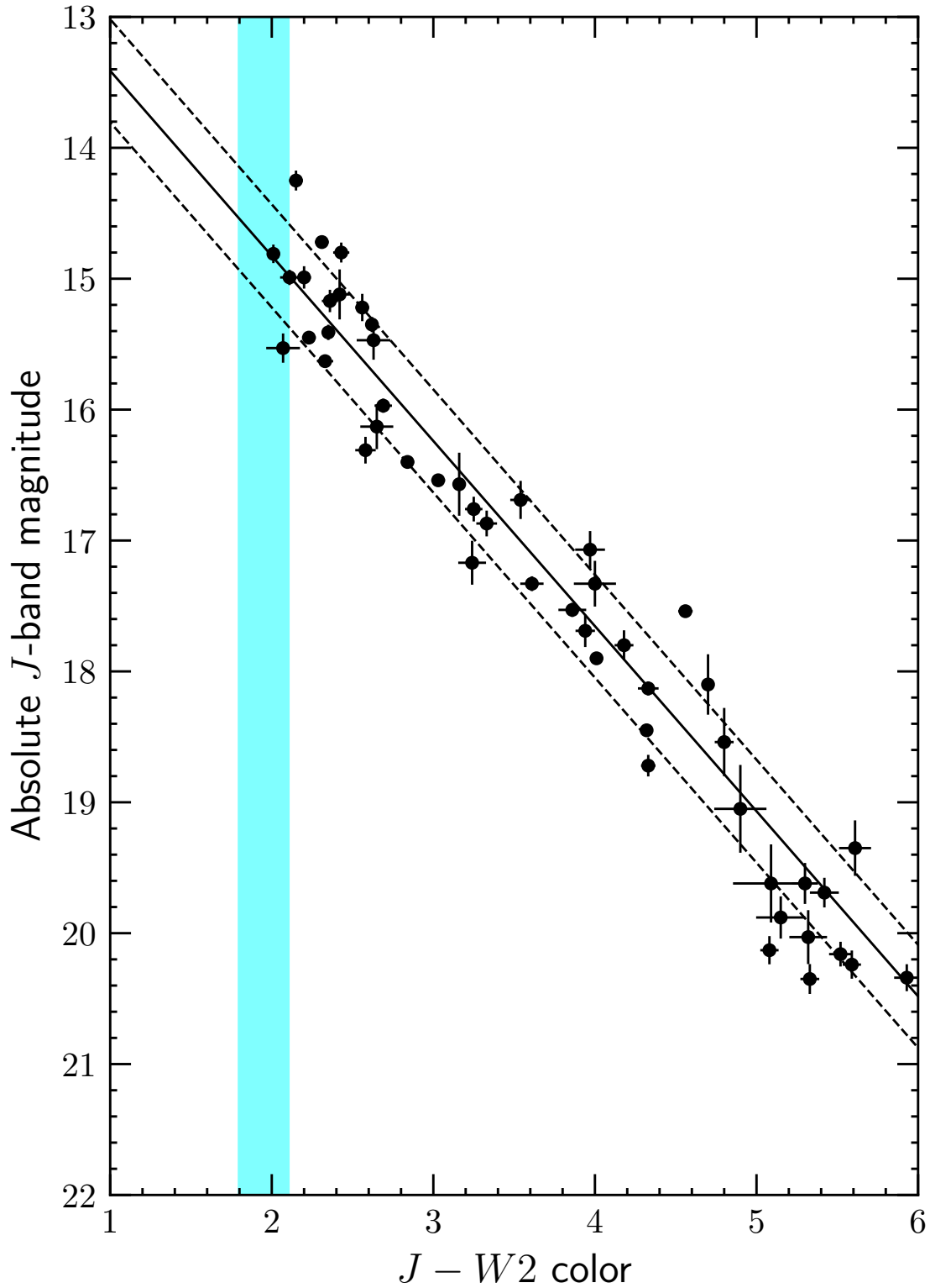
Figure 9. NIR color-magnitude diagram for cold brown dwarfs (class T and Y). Black points are taken from the homogenized dataset on late T-dwarfs and Y dwarfs presented by Leggett et al. (2017). The solid black line is a linear fit to the points. The dashed black lines are parallel to the solid line, and are offset by one standard deviation between the fit and the data points. The cyan shaded region shows the constraint on BDR J1750+3809’s NIR colors from Table 1
