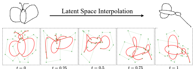
Figure 7. Interpolating between two sketches by walking on the latent space as: \mathbf{z} = \mathbf{z}_{butterfly} \cdot (1 - t) + \mathbf{z}_{mosquito} \cdot t
