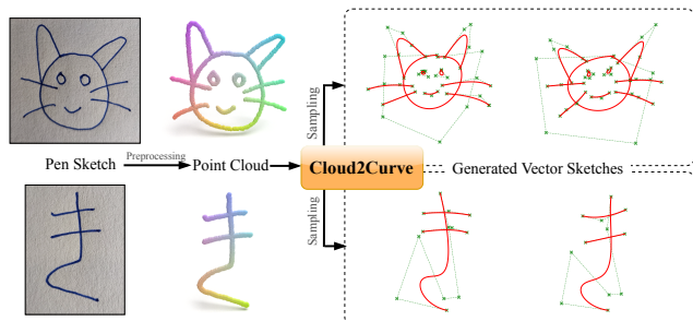
Figure 1. Cloud2Curve capability teaser. Top: Our trained model can vectorize a pen-on-paper sketch using scalable parametric curves. Bottom: Cloud2Curve can be trained on raster datasets such as KMNIST, where existing generative models cannot.
