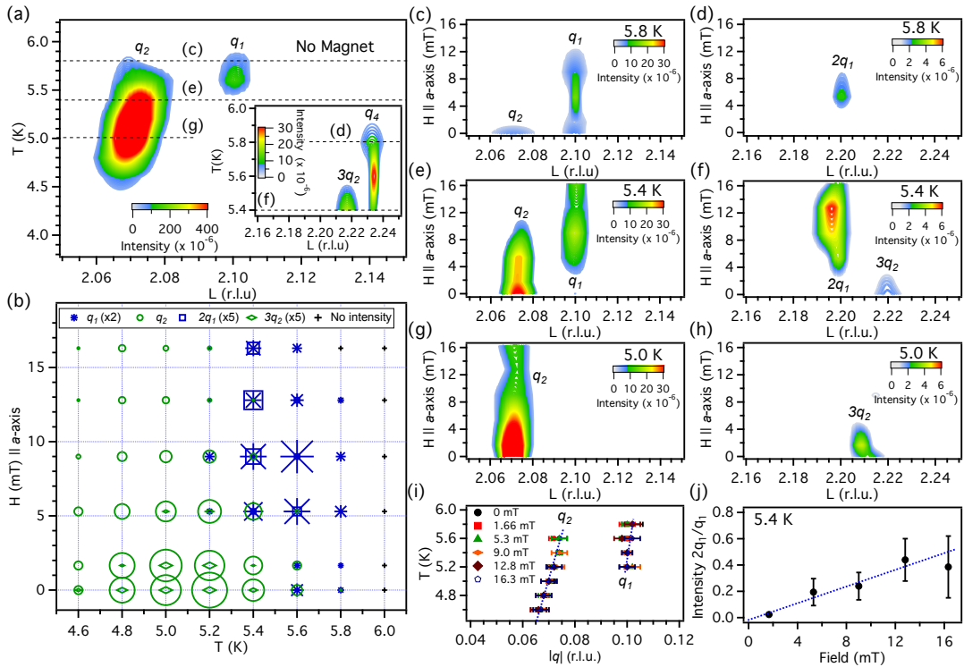
FIG. 2: (a) Colourscale image of the normalised magnetic resonant X-ray scattered intensity as a function of T and reciprocal lattice co-ordinate (0,0,L) in zero field (no magnet). Inset, the corresponding intensity at wavevectors q_4 and 3q_2 . (b) H - T phase diagram of the integrated intensity at q_1 , q_2 , 2q_1 and 3q_2 for H applied along the a -axis. The marker size is proportional to the normalised integrated intensity (scaling is shown in the legend). Measured points where no intensity is found are marked by crosses. The data at zero field in this plot are with the magnet in place. (c)-(h) Colourscale maps of scattered intensity as a function of H along a -axis and (0,0,L) for 5.8, 5.4 and 5.0 K (the corresponding temperatures at zero field are marked by dashed lines in (a)). (i) T dependence of q_1 and q_2 . Points at different field superimpose. Dashed lines are guides to the eye showing that both q_1 and q_2 increase linearly with temperature. (j) The ratio of integrated intensity between the second harmonic 2q_1 and q_1 at 5.4 K as a function of field. The dashed line is a guide to the eye.
