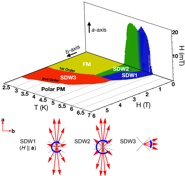
FIG. 4: The schematic H_a - H_b - T phase diagram for PrPtAl with fields applied along the easy a -axis (vertical) and hard b -axis (horizontal), based on our measurements. SDW1 (Blue), SDW2 (green) and SDW3 (Red) modulated states form a ridge around the first order FM plane (yellow) across which the FM moment \mathbf{M} \parallel \mathbf{a} reverses. The phase boundaries between the different modulated states and on the low-field low-temperature side of the ridge are first order. Schematics of the moment directions viewed along the c -axis for one modulation period for the different modulated states SDW1, SDW2 and SDW3 are shown below the phase diagram.
