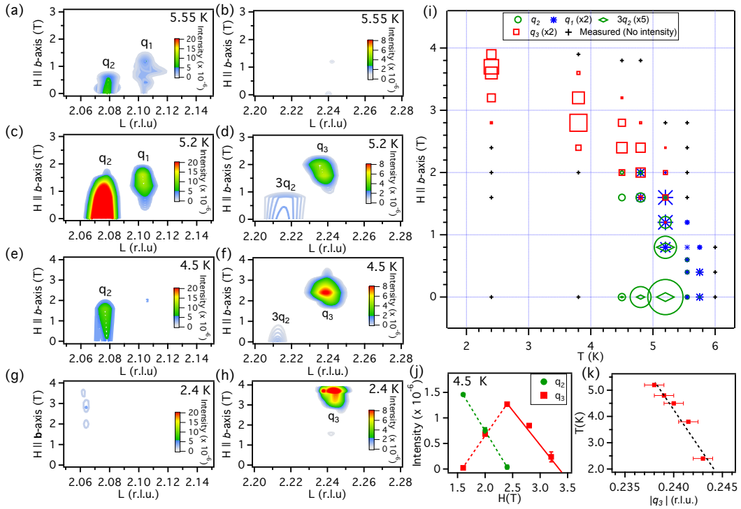
FIG. 1: Colourscale images of normalised magnetic resonant X-ray scattered-intensity as a function of field ( H ) applied along the b -axis and scattering vector (0,0,L) at (a) and (b) 5.55 K, (c) and (d) 5.2 K, (e) and (f) 4.5 K and (g) and (h) 2.4 K. Scattering at wavevectors q_1 and q_2 , survives up to 2 T, before abruptly being replaced by scattering at wavevector q_3 . (i) The H - T phase diagram showing the integrated intensity at q_1 , q_2 , q_3 and 3q_2 up to 4 T. The marker size is proportional to the integrated intensity (scaling shown in the legend). Measured points where no intensity was found are marked by crosses. (j) The variation in integrated intensity at q_2 and q_3 with H at 4.5 K. (k) T dependence of the magnitude of q_3 (the dashed line is a guide to the eye).
