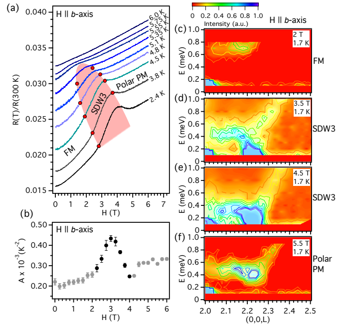
FIG. 3: (a) The MR, normalised to the zero field resistivity value at 300 K, for field applied along the b -axis. The region where SDW3 exists is shaded red, with markers showing the transition field seen in X-ray scattering. (b) The A coefficient of resistivity for Fermi liquid fits between 4-2.2 K as a function of field. Black markers correspond to the region where SDW3 exists within this temperature range. (c)-(f) Colourscale images of inelastic neutron scattered intensity (in arbitrary units) as a function of energy transfer and reciprocal lattice co-ordinate (0, 0, L) at 1.7 K for different fields applied along the b -axis. These show the dispersion of the lowest energy magnetic excitation at (c) 2 T in the FM state, (d) 3.5 T and (e) 4.5 T in the SDW3 state and (f) 5.5 T in the polar PM state.
