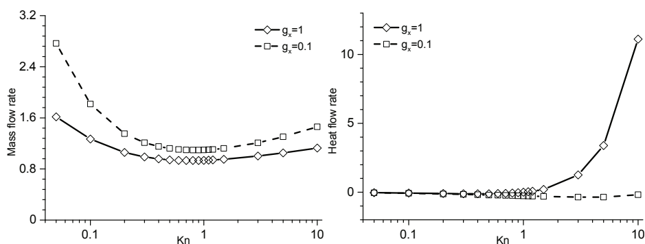
Figure 8: Mass and heat flow rates for force-driven Poiseuille flows of over a range of Kn . Both fluid quantities are re-normalized by the force magnitude.
