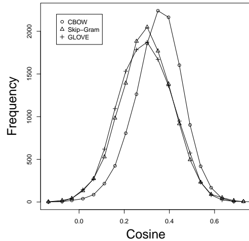
Figure 4: Frequency against Cosine.
