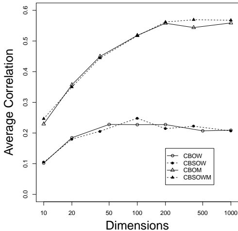
Figure 5: Average Correlation on Noun-Verb Evaluation Task against Size of Representations.
