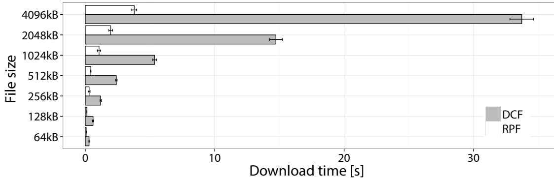
Figure 8: WLAN with 2 stations: one downloads small-sized files from the AP using HTTP over a link operating at 54Mb/s; the other is backlogged and uploads to the AP using TCP over a 6Mb/s link. Download time of different-size objects with DCF and the proposed RPF scheme. Experimental data.
