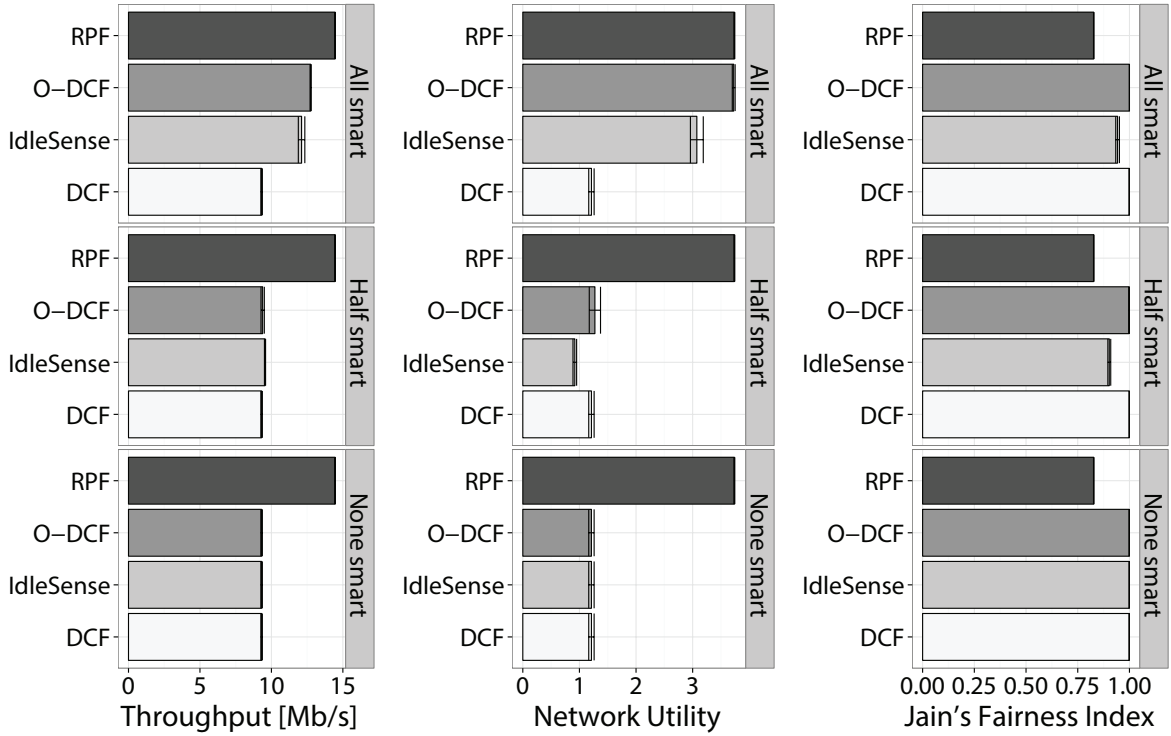
Figure 11: WLAN with 8 backlogged stations transmitting using UDP. Stations use the OFDM PHY layer (802.11a), fully heterogeneous bit rates and employ our proposal (RPF), Idle Sense, O-DCF, and standard DCF. Total throughput (left), network utility (centre), and Jain's fairness index (right) in three scenarios: all clients smart (implementing changes as required, top), half smart (middle), and respectively all legacy (none smart, bottom). Simulations results.
