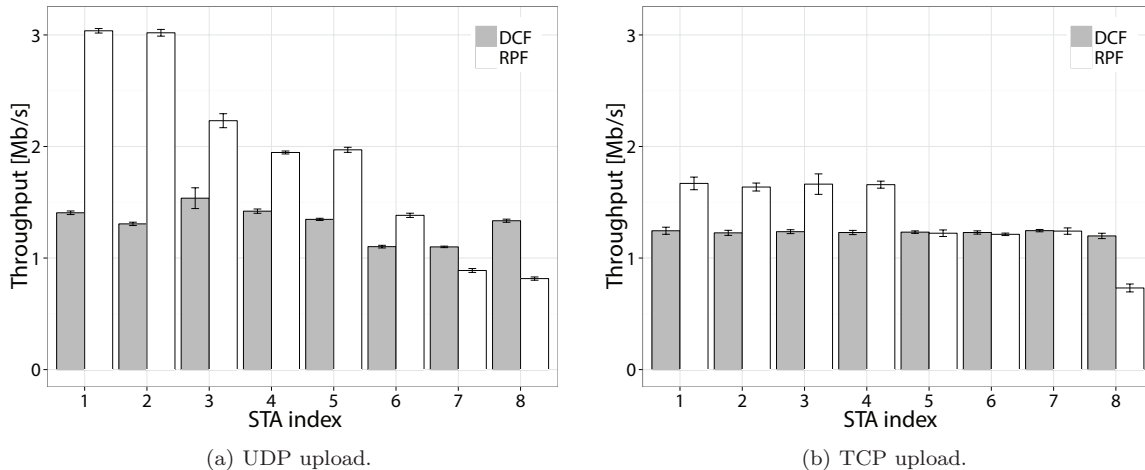
Figure 5: WLAN with 8 backlogged stations sending 1400-byte packets to the AP. Each station uses the OFDM PHY layer (802.11a) and transmits using a different MCS. Individual throughput performance with standard DCF configuration and the proposed proportional-fair (RPF) allocation scheme over UDP (left) and TCP (right). Experimental data.
