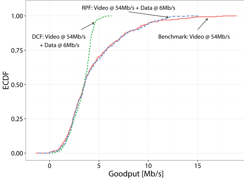
Figure 7: WLAN with 2 stations: one streams MP4 video from the AP over a wireless link operating at 54Mb/s; the other sends backlogged uplink TCP traffic at 6Mb/s PHY bit rate. Empirical CDF of the goodput attained by the video stream alone and with competing traffic, when the AP operates with legacy DCF and respectively with the proposed RPF scheme. Experimental data.
