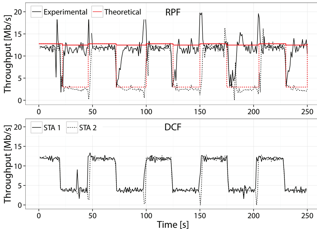
Figure 9: WLAN with 2 backlogged stations sending UDP traffic to the AP. STA 1 always operates at 54Mb/s. STA 2 alternates its bit rate between 54 and 6 Mb/s every 25 seconds. Time evolution of the individual throughputs with both DCF and the proposed RPF scheme. Experimental data vs theoretical optimum prediction.
