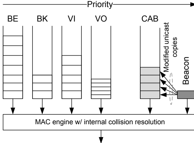
Figure 2: Software queues exposed by mac80211 and the implementation principle behind the proposed unicast beaming mechanism. A copy of the broadcast beacon is made for each client, updated with the corresponding destination address and CW settings, and placed on the CAB queue.
