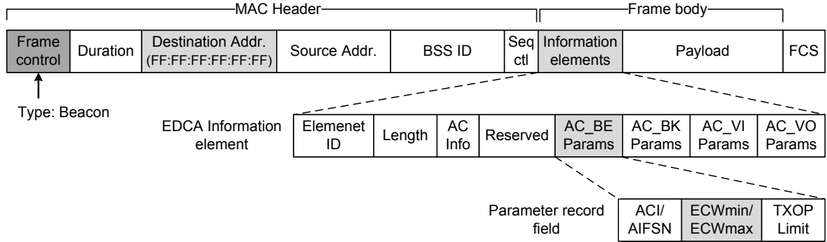
Figure 3: Structure of a beacon management frame. Fields modified to generate unicast beacons that configure individual clients are highlighted. The destination address field is changed from broadcast to that of the target station. ECWmin and ECWmax settings are updated with the values that solve utility maximisation.
