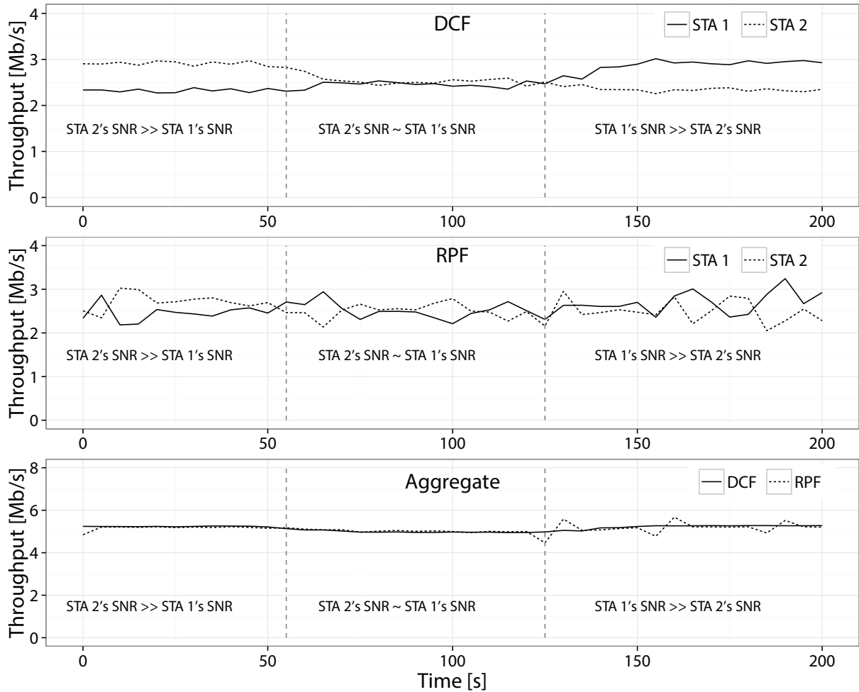
Figure 10: WLAN with 2 stations sending at 6Mb/s. STA 1 uses fixed TX power (16dBm). STA 2 starts with maximum supported power (30dBm) and reduces this gradually down to the minimum (0dBm). Time evolution of individual throughputs with DCF (top), the proposed RPF scheme (middle), and the aggregate network throughput in both scenarios (bottom). Experimental data.
