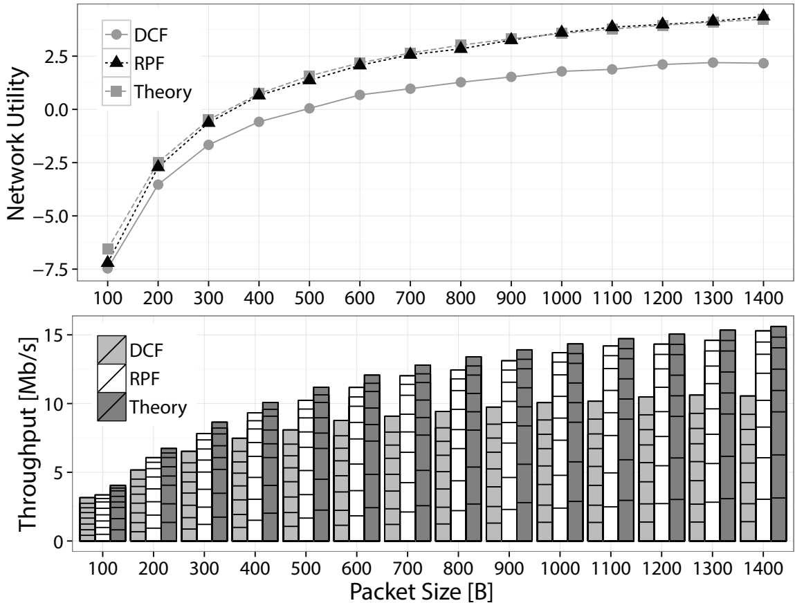
Figure 6: WLAN with 8 backlogged stations transmitting to the AP using UDP. Stations use the OFDM PHY layer (802.11a) and fully heterogeneous bit rates. Network utility (top) and individual/total throughput (below) with standard DCF configuration and the proposed proportional-fair (RPF) allocation scheme as the packet size is varied. Experimental data vs. theoretical optimum prediction.
