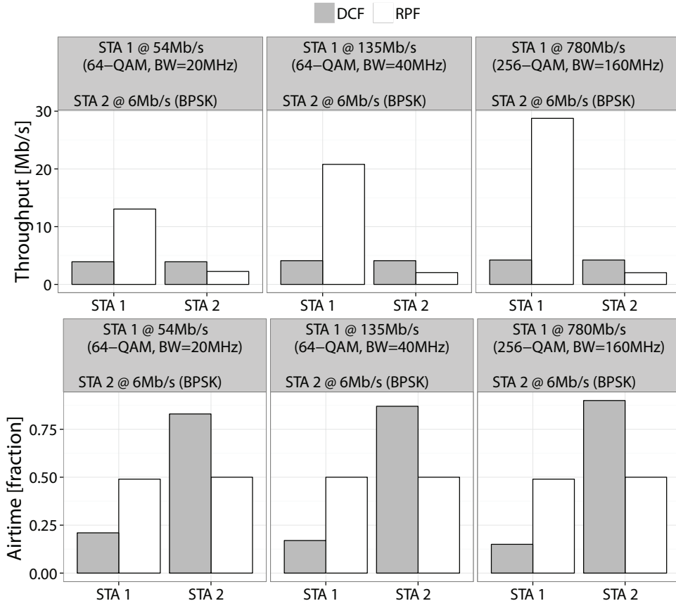
Figure 1: WLAN with 2 backlogged stations sending 1000-byte packets. STA 2 transmits at 6Mb/s (BPSK) on a 20MHz channel. STA 1 transmits at 54Mb/s (20MHz channel, 64-QAM), 135Mb/s (40MHz channel, 64-QAM), and respectively at 780Mb/s (160MHz channel, 256-QAM). Individual throughput (above) and airtime (below) with DCF (dark bars) and respectively with the proposed rigorous proportional-fair (RPF) allocation scheme (light bars). Analytical model.
