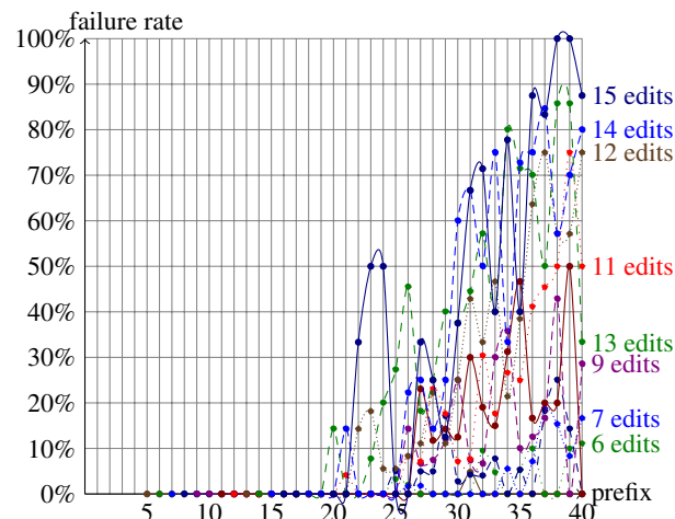
Figure 2: Ratio of prefix matching processes abandoned due to exceeding the 100ms time limit (showing only curves with a minimum of 5 edits).
