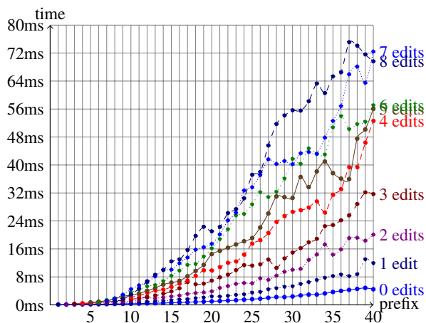
Figure 1: Average response time of baseline method based on length of the prefix and number of edits: The main bottleneck is the string edit distance between prefix and path.
