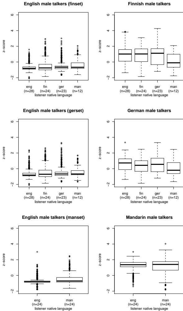
Fig. 2. Boxplot of listeners’ z-scores per native language for male talkers. (See caption for Figure 1 for abbreviations.)
