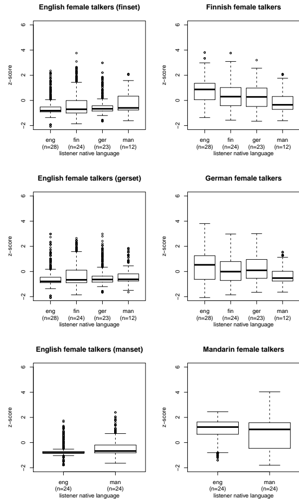
Fig. 1. Boxplot of listeners’ z-scores per native language for female talkers. ‘n’ = number of listeners, ‘eng’ = English, ‘fin’ = Finnish, ‘ger’ = German, ‘man’ = Mandarin, ‘finset’ = Finnish/English set, ‘gerset’ = German/English set & ‘manset’ = Mandarin/English set (Experiments I and II).
