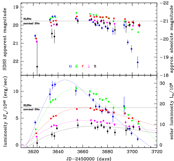
FIG. 2.— Light curves of PSN 000123+000504. Top panel: The SN extinction-corrected observed magnitudes in the AB magnitude system and the approximate absolute magnitudes (host extinction and K -corrections not included) for five SDSS filters (marked with colors). For clarity, data points are shifted by -0.8 ( u -band), -0.4 ( g -band), +0.4 ( i -band), +0.8 ( z -band) days with respect to the observed date. The horizontal dashed line marks the division between normal SNe and SLSNe from Gal-Yam (2012). Bottom panel: The absolute magnitudes from the top panel converted to luminosity. The SN peaked above 10^{44} erg/s, typical for SLSNe and atypical for normal SNe. The combined peak luminosity from five filters exceeded 3.5 \times 10^{44} erg/s (Table 3).
