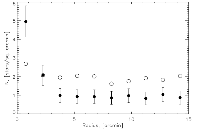
Fig. 5. Radial density distribution for stars in the field of Koposov 52. Solid circles represent the density of the stars lying closely to the isochrone. Open circles denote the density of the field stars lying far from the isochrone.
