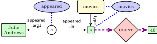
(a) Ungrounded Graph
