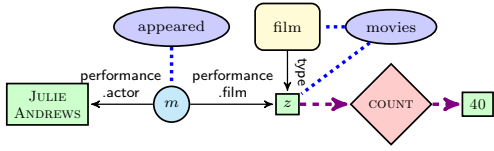
(c) Grounded graph
