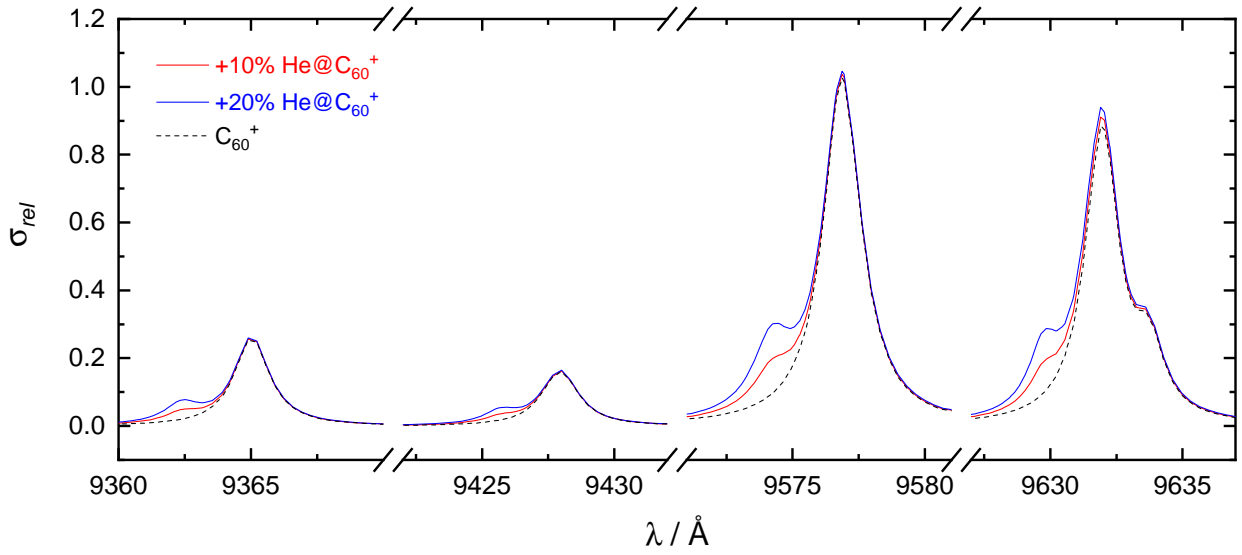
Fig. 5.— Absorption band profiles of C_{60}^+ (black), and He@ C_{60}^+ : C_{60}^+ mixtures in ratios 0.1:1 (red) and 0.2:1 (blue). The data are from the fits shown in Figure 4 with wavelengths shifted to take into account the perturbation caused by the weakly bound Helium atom.
