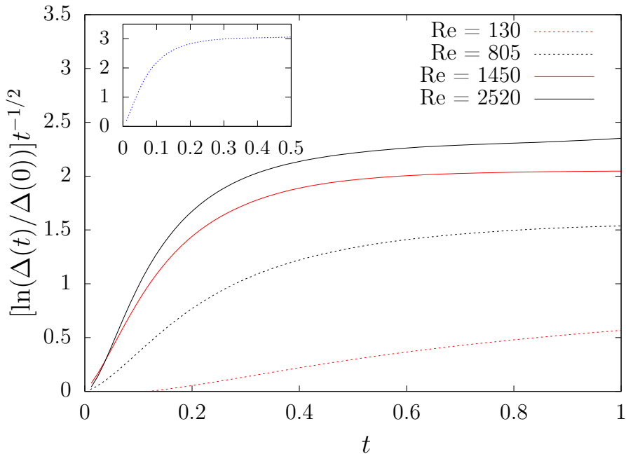
Figure 2: The nonlinear amplifications of perturbations for different Reynolds numbers Re = 130, 805, 1450, 2520, 6210 before their nonlinear saturations. The case for Re = 6210 is shown in the upper left corner inset. \Delta(t) is the energy norm defined in (2.4). The horizontal portions of the curves represent amplifications of e^{c\sqrt{t}} in t as we predicted in (1.1).
