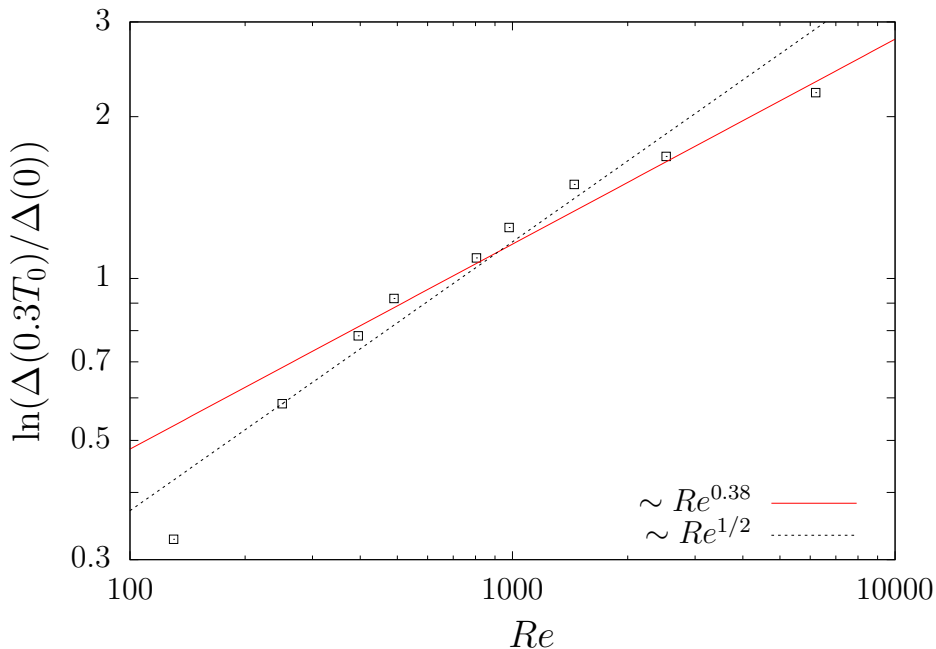
Figure 4: The Reynolds number dependence of the nonlinear amplifications of perturbations up to the time t = 0.3T_0 , where T_0 is the large eddy turnover time which is around 2. \Delta(t) is the energy norm defined in (2.4). The dashed curve is a fit to \sim \sqrt{Re} , and the red (grey) curve is a fit to \sim Re^{0.38} . Both the horizontal and vertical axes are in logarithmic scales.
