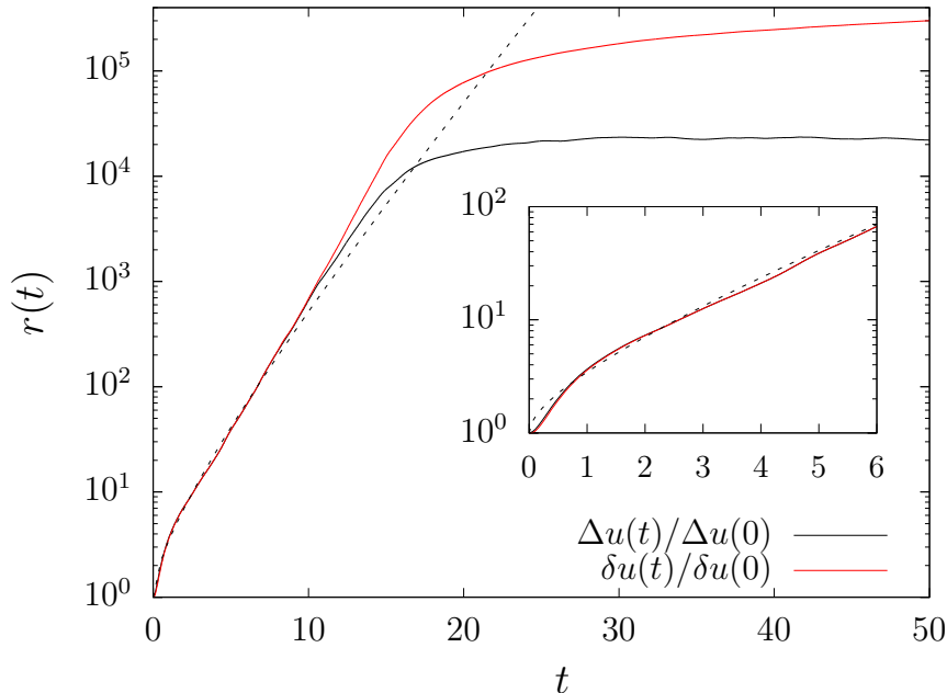
Figure 1: The divergence of the linear amplification and the nonlinear amplification of a perturbation with initial energy norm \Delta u(0) = \delta u(0) = 0.01 (2.4)-(2.5) and the Reynolds number Re = 230 . The vertical axis symbol r(t) represents either \frac{\Delta u(t)}{\Delta u(0)} or \frac{\delta u(t)}{\delta u(0)} . Divergence and nonlinear saturation happens around t = 10 which is about 5 large eddy turnover time 5T_0 . The inset zooms in the time interval t \in [0, 6] . The dashed line is the fitting curve 0.9\sqrt{t} + 0.34t of the type in the exponent of our estimate (1.1).
