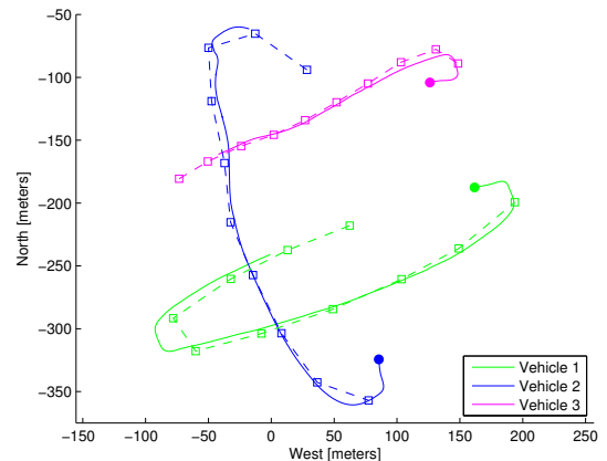
Fig. 5. Paths travelled by each vehicle (6 minutes of the 70 minute mission). The smooth line represents the GPS position of each vehicle, with the current location indicated by a circle. The dashed line segments illustrate the estimated path as reconstructed using a multi-vehicle EKF as described in Section V. The covariance of the estimated path is omitted for clarity. With a data transmission every 10 seconds and keyframes spaced every 4 transmissions, each multi-vehicle pose update is spaced 40 seconds apart. Note also that the reconstructed pose lags the current position by approximately 30-40 seconds in this figure. See Section VI-A.
