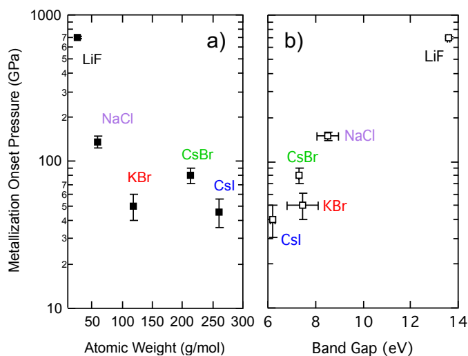
FIGURE 4. The onset of high reflectivity as a function of atomic weight (a) and electronic band gap [18] at ambient pressure (b) (LiF from [15]).
