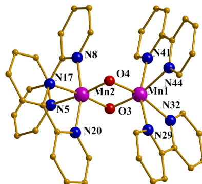
Fig. 1. The molecular structure of the complex cation in 1 ·3CH 3 CN and 2 ·2CH 3 CN·1H 2 O. Colour scheme: Mn = violet, C = gold, O = red, N = blue. Counter ions, H atoms and solvent molecules omitted for clarity.
