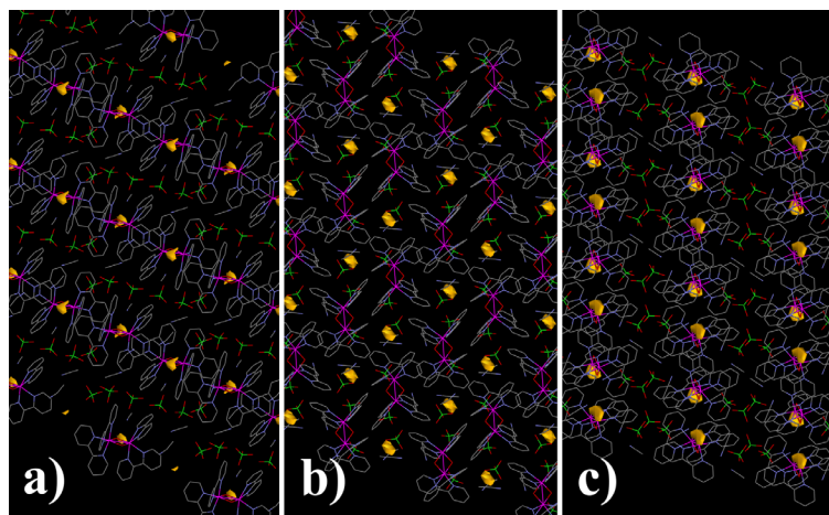
Fig. 5. Void diagrams of 1 ·3CH 3 CN along the three crystallographic axes a , b and c at 2.00 GPa. Probe size: 0.8 Å.
